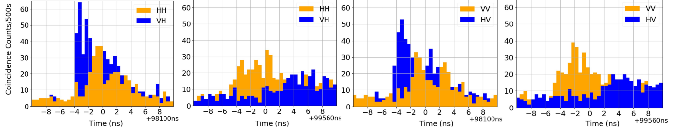
Fig. 4. Coincidence counts distributions, first-row plots with narrow-band photon pairs at (1574, 1557.51) nm, second-row plots with broadband photon pairs. The first and third column plots represent destination-2 measurements, around 98100 ns delay. The second and fourth column plots represent destination-1 measurements, around 99560 ns delay.
