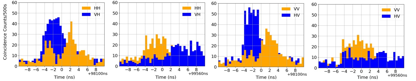
Fig. 5. Coincidence counts distributions, first-row plots with narrow-band photon pairs at (1584, 1547.51) nm, second-row plots with broadband photon pairs. The first and third column plots represent destination-2 measurements, around 98100 ns delay. The second and fourth column plots represent destination-1 measurements, around 99560 ns delay.
