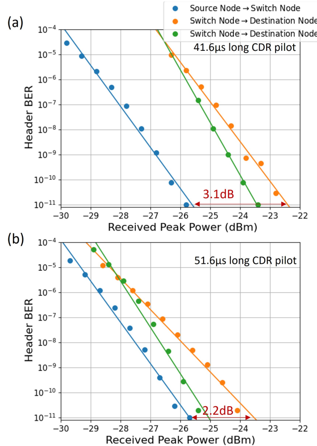
Fig. 9. Header BER measured at QWSR at the core (blue traces) and at the edges (orange and green traces) vs. received peak power for (a) 41.6 \mu\text{s} and (b) 51.6 \mu\text{s} long CDR pilot sequence.
