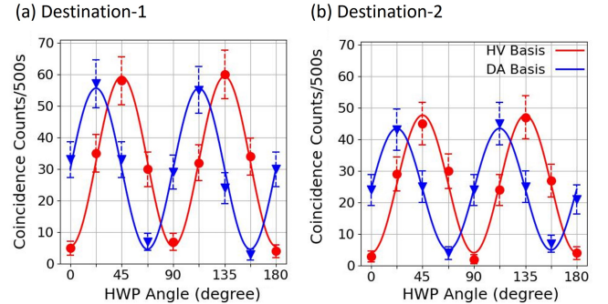
Fig. 7. Coincidence counts per 500 seconds with varying half-wave plate angle at (a) destination-1 and (b) destination-2 quantum receivers.
