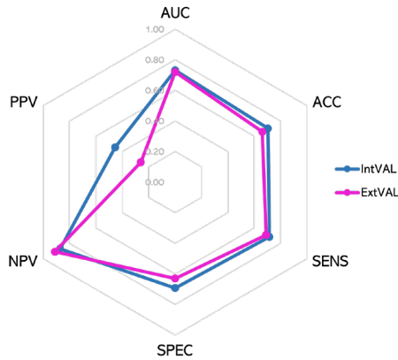
Fig. 2. Performance's radar graph on validation sets.
