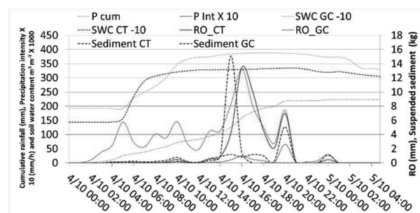
Figure 2. Cumulative precipitation (P cum, mm), Precipitation intensity (P int, X10, mm), runoff (RO, mm), soil water content (SWC, m 3 m -3 X1000) and suspended sediment (kg) in CT and GC.
