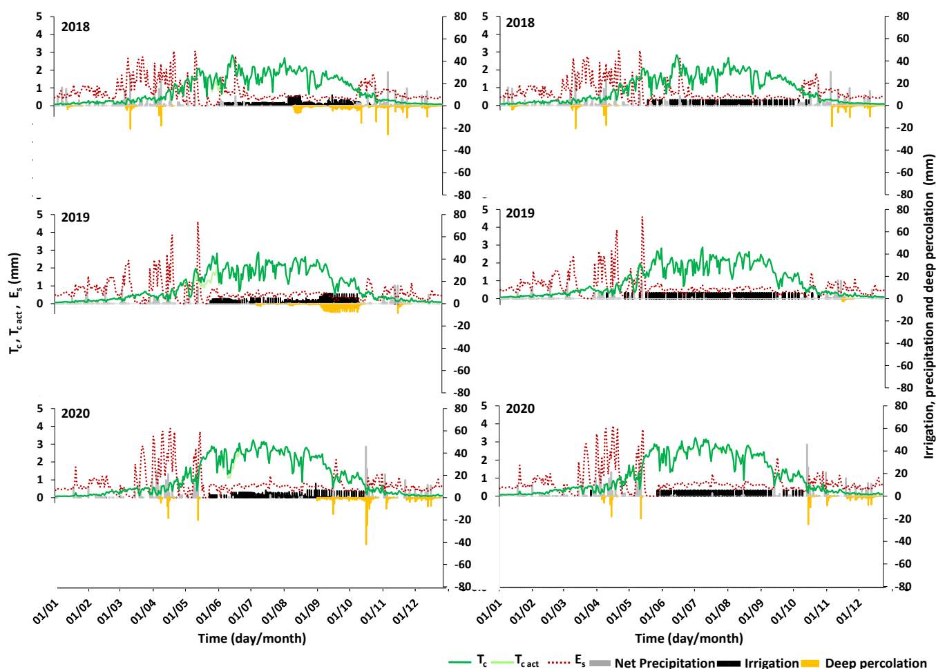
Figure 8. Daily evolution of the potential crop transpiration ( T_c ), actual crop transpiration ( T_{c\text{ act}} ), soil evaporation ( E_s ), and deep percolation rates at Samora Correia vineyard as monitored in the field (left) and after optimization of the irrigation schedules (right) during 2018–2020.
