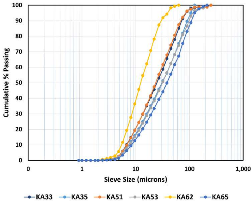
Figure 35. Particle size distribution for garnet from the old tailings storage facility (n=6).
