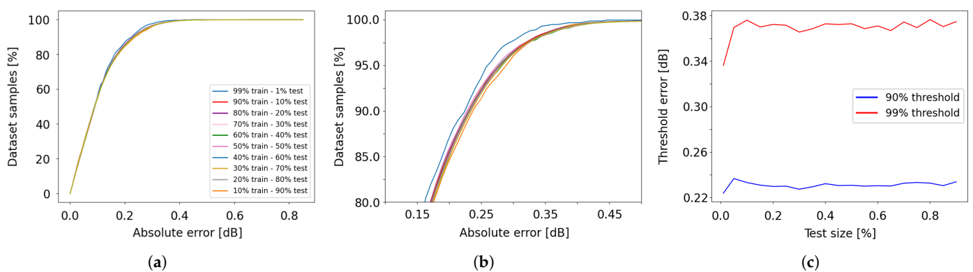
Figure 20. Cumulative distribution of the absolute error for the L-band EDFA device, as a function of the train/test split ratio. (a) Overview of absolute errors; (b) Zoomed-in view of the y-axis region between 80% and 100%; (c) 90% and 99% error thresholds versus test size.
