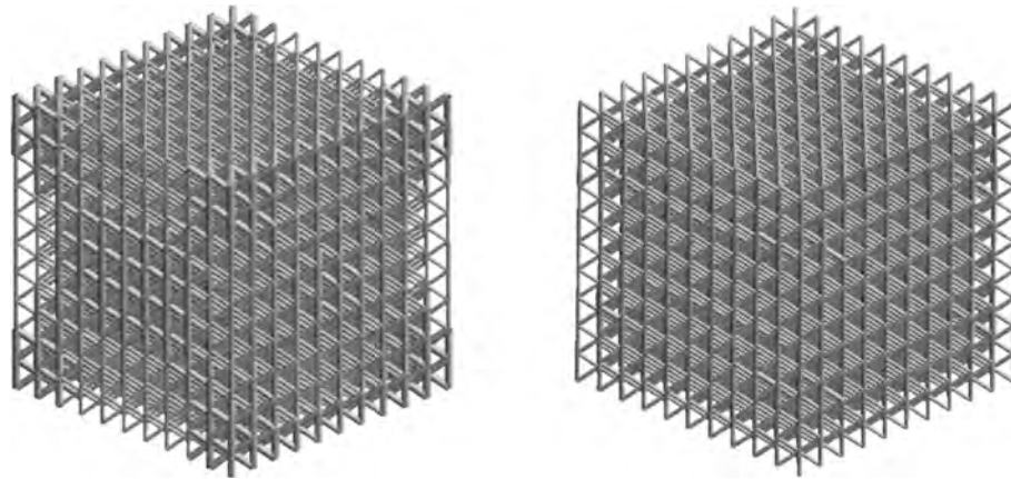
Fig. 8. Bccz1 and bccz2 graded samples (using threshold 3).
