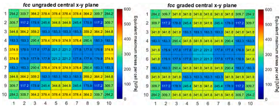
Fig. A4. Map of the maximum equivalent stresses registered per cell concerning ungraded (left) and graded (right) fcc samples.
