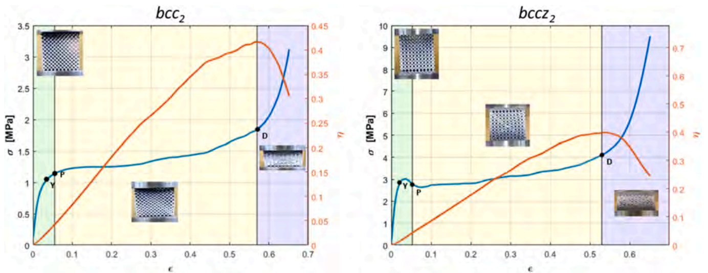
Fig. 19. Stress–strain diagrams for bcc2 (left) and bccz2 (right) with relevant points: yield, begin of the plateau and densification.
