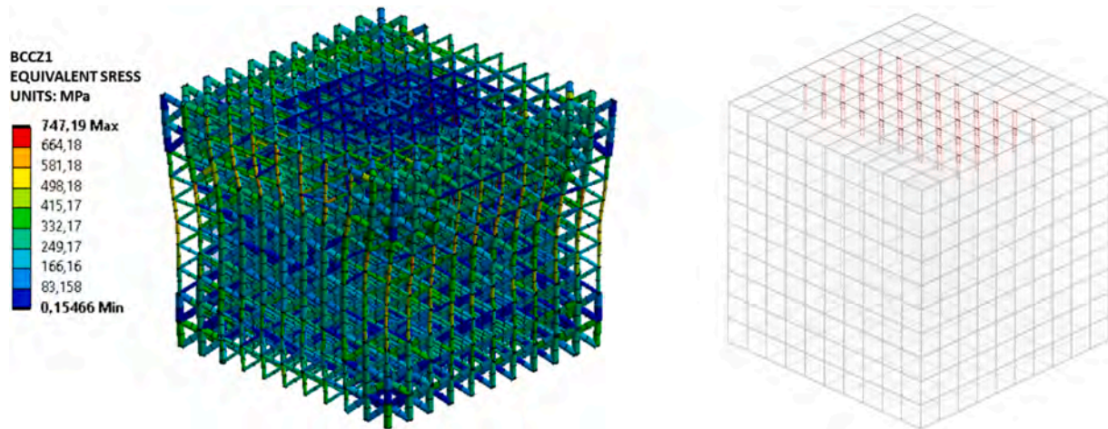
Fig. 11. Representation of equivalent stress distribution for bccz1 (left) and relative equivalent stress concentration scheme (right).
