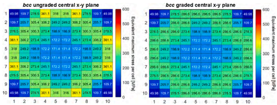
Fig. A2. Map of the maximum equivalent stresses registered per cell concerning ungraded (left) and graded (right) bcc samples.
