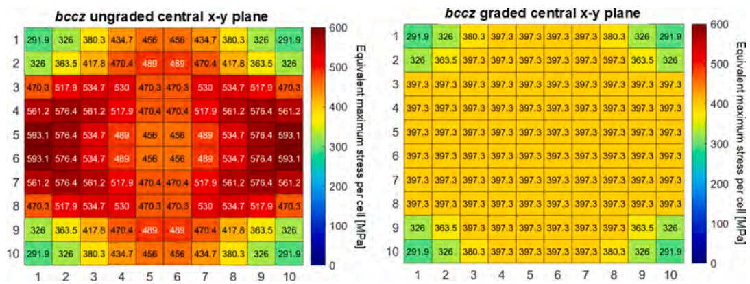
Fig. A3. Map of the maximum equivalent stresses registered per cell concerning ungraded (left) and graded (right) bcc samples.
