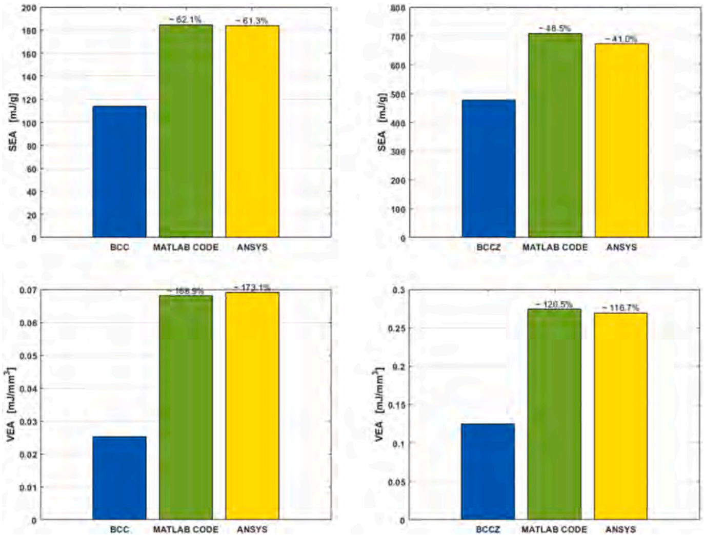
Fig. 13. SEA and VEA for bcc (left) and bccz (right) histograms, respectively for the initial configuration (blue), the graded via process 1 configuration with SEA and VEA evaluated via Matlab (green) and the graded via process 1 configuration with SEA and VEA evaluated via FEM (yellow).
