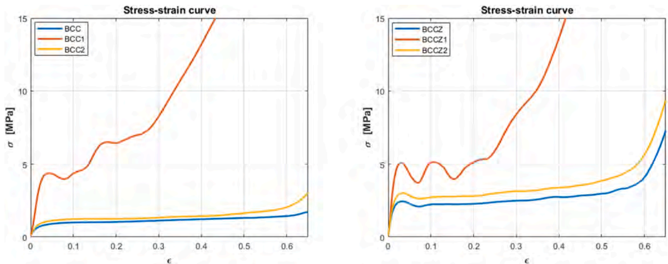
Fig. 16. Averaged stress–strain diagrams for bcc (left) and bccz (right) ungraded and graded samples from experimental compression tests.
