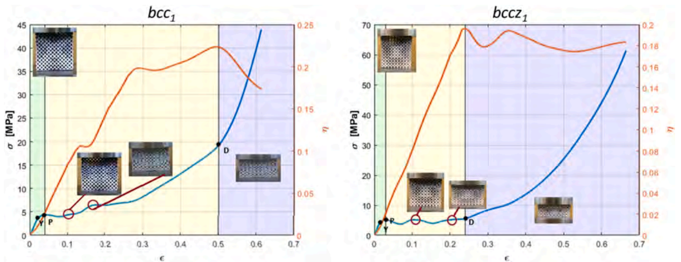
Fig. 18. Stress–strain diagrams for bcc1 (left) and bccz1 (right) with relevant points: yield, begin of the plateau and densification.
