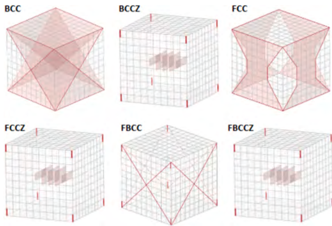
Fig. 6. Equivalent stress concentration schemes for all of the ungraded samples.
