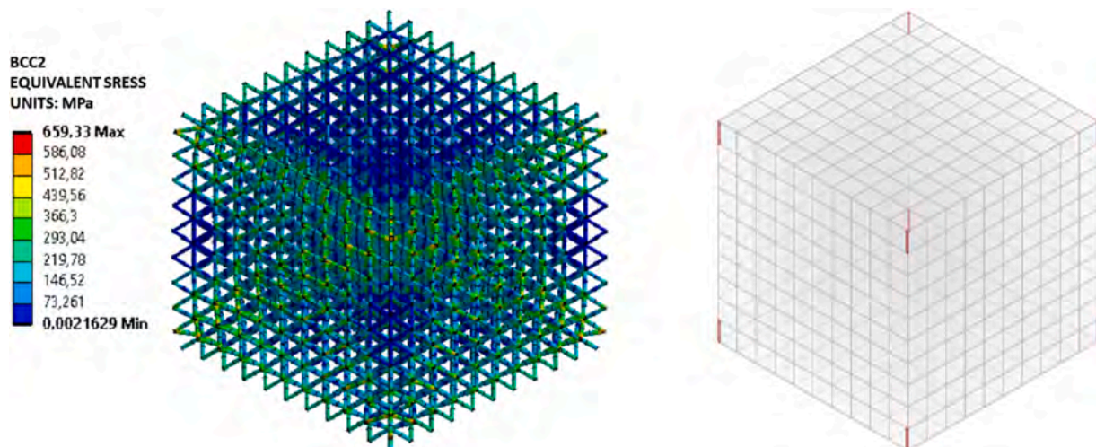
Fig. 10. Representation of equivalent stress distribution for bcc2 (left) and relative equivalent stress concentration scheme (right).
