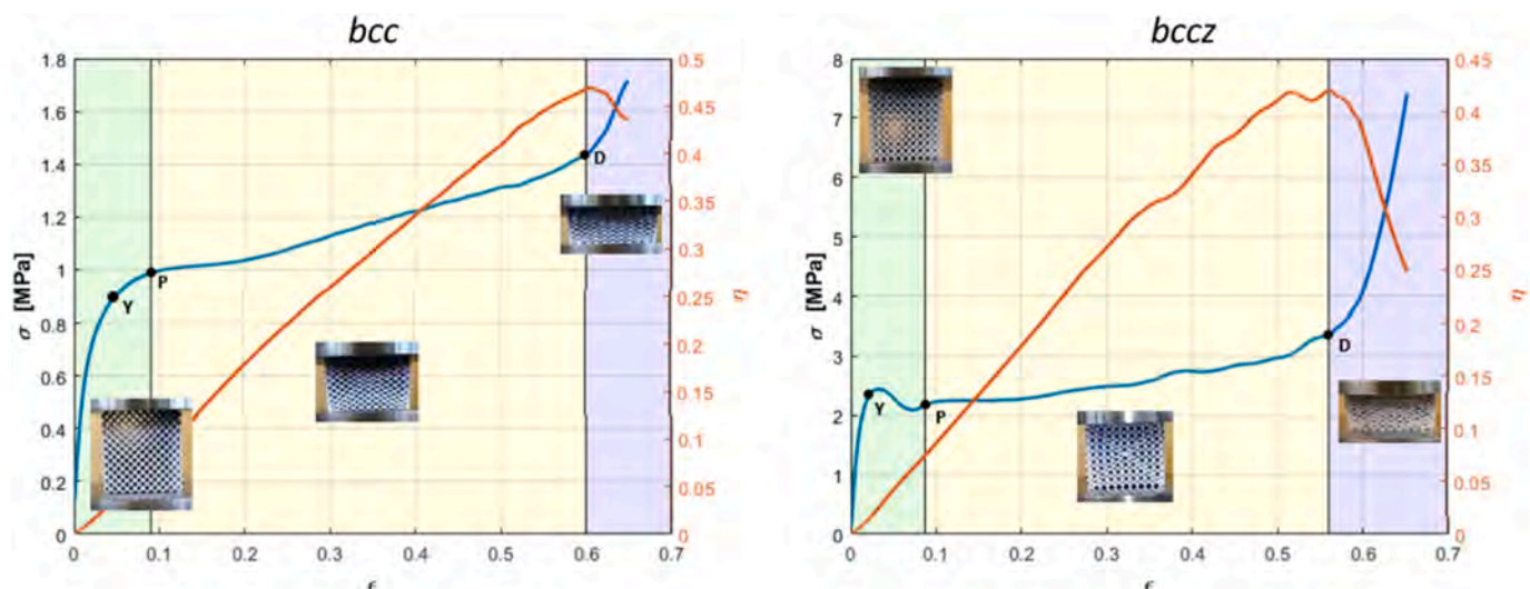
Fig. 17. Stress–strain diagrams for bcc (left) and bccz (right) with relevant points: yield, begin of the plateau and densification.
