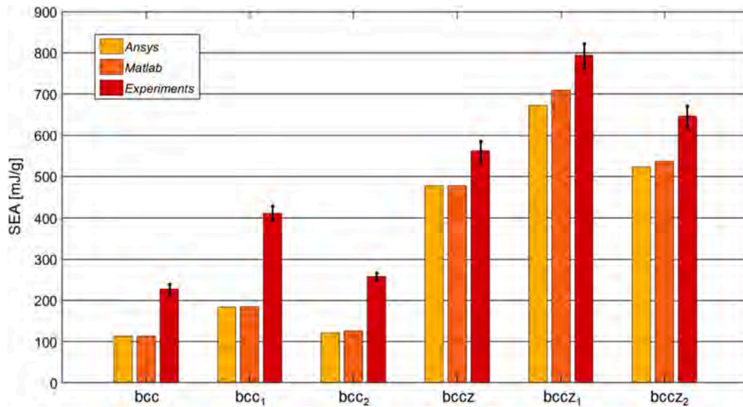
Fig. 20. SEA values extracted from Ansys FEM simulations, Matlab and Experimental tests for all of the samples considered for the experimental validation.
