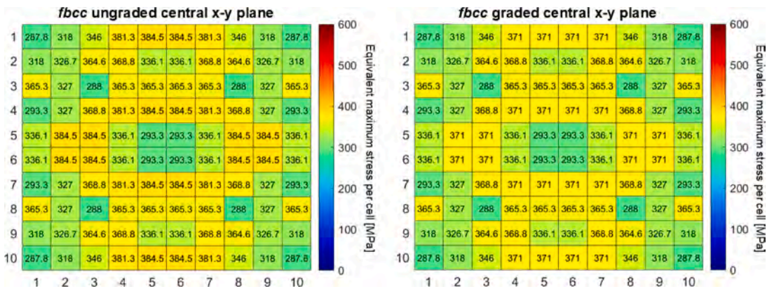
Fig. A6. Map of the maximum equivalent stresses registered per cell concerning ungraded (left) and graded (right) fbcc samples.
