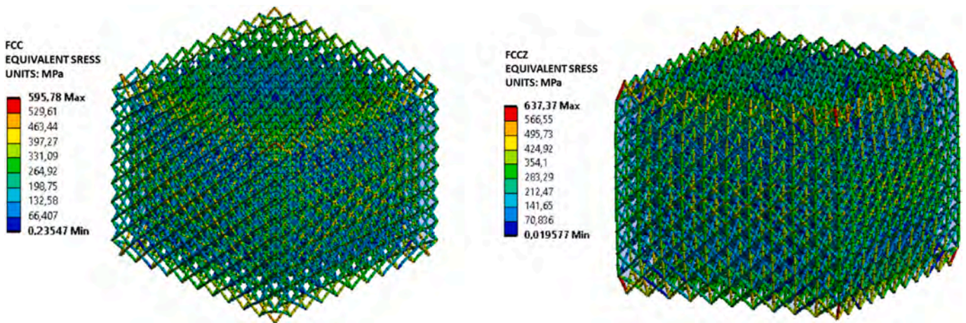
Fig. 4. Representation of equivalent stress distribution for ungraded samples fcc (left) and fccz (right) from Ansys.
