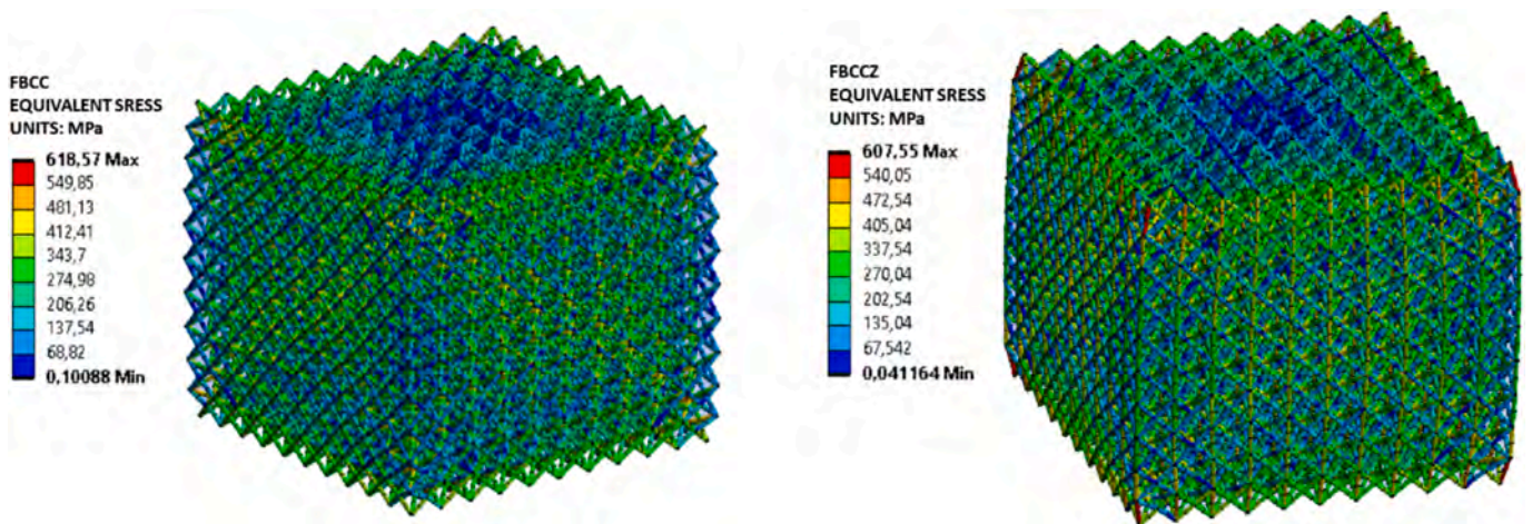
Fig. 5. Representation of equivalent stress distribution for ungraded samples fbcc (left) and fbccz (right) from Ansys.
