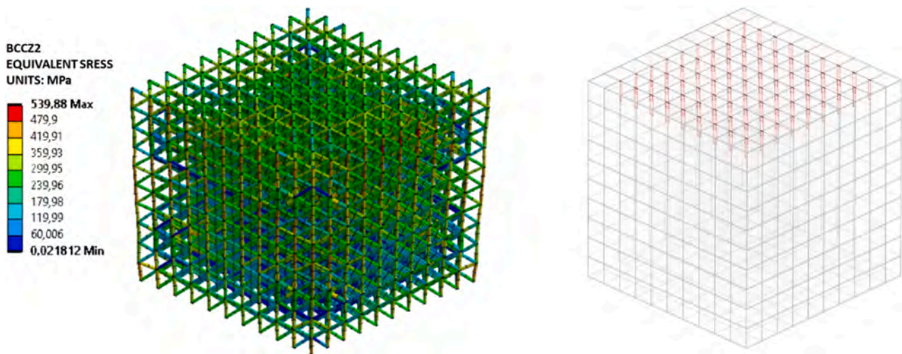
Fig. 12. Representation of equivalent stress distribution for bccz2 (left) and relative equivalent stress concentration scheme (right).
