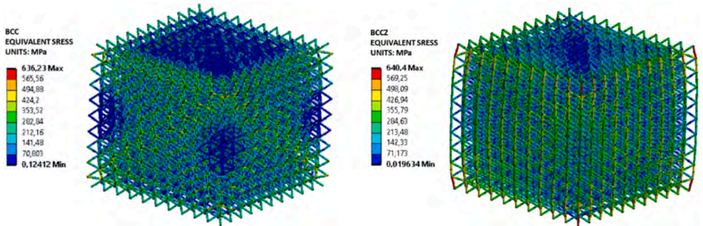
Fig. 3. Representation of equivalent stress distribution for ungraded samples bcc (left) and bccz (right) from Ansys.
