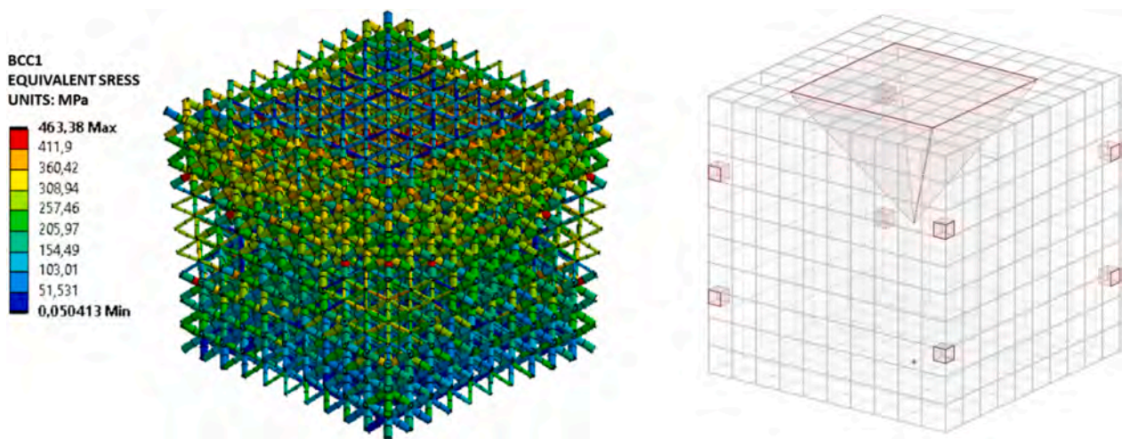
Fig. 9. Representation of equivalent stress distribution for bcc1 (left) and relative equivalent stress concentration scheme (right).
