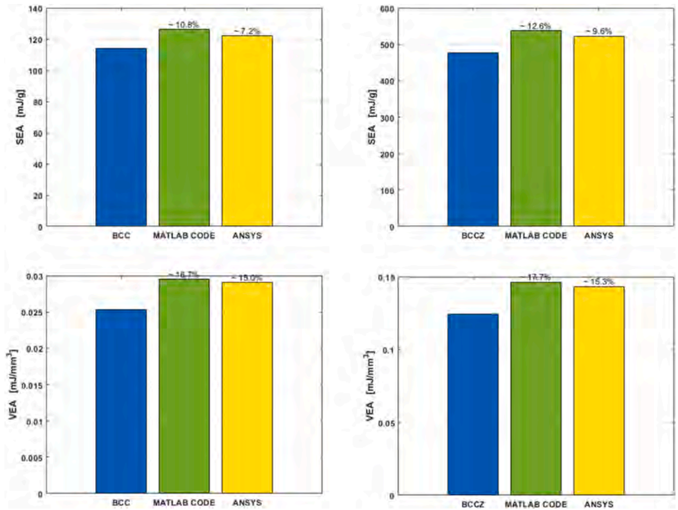
Fig. 14. SEA and VEA for bcc (left) and bccz (right) histograms, respectively for the initial configuration (blue), the graded via process 2 configuration with SEA and VEA evaluated via Matlab (green) and the graded via process 2 configuration with SEA and VEA evaluated via FEM (yellow).
