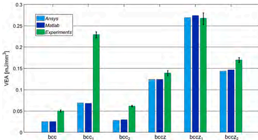
Fig. 21. VEA values extracted from Ansys FEM simulations, Matlab and Experimental tests for all of the samples considered for the experimental validation.
