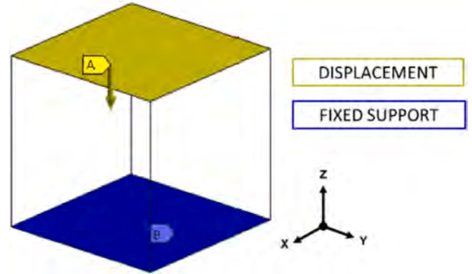
Fig. 2. Graphical representation of the boundary and load conditions applied to the samples for the FEM simulations.
