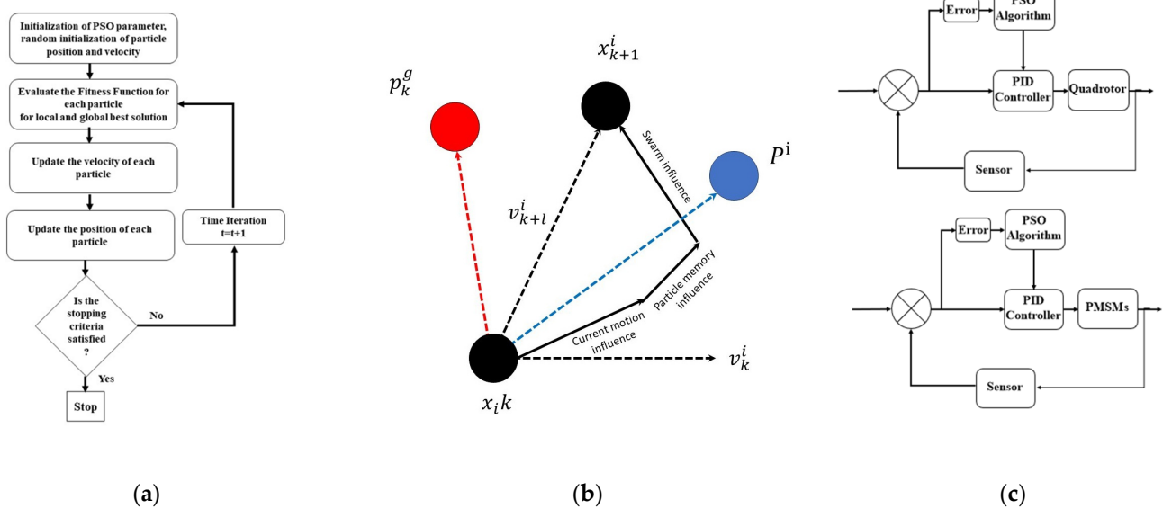
Figure 2. (a) Flow chart of the PSO algorithm based on [19]; (b) Process of searching for a new position in the PSO methodology; (c) Schematic representation of how the PSO framework is used for optimizing the PID parameters of both quadrotor and PMSMs' controllers.
