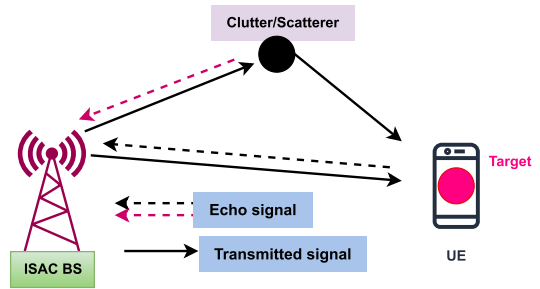
FIGURE 14. Mono-static ISAC system.
