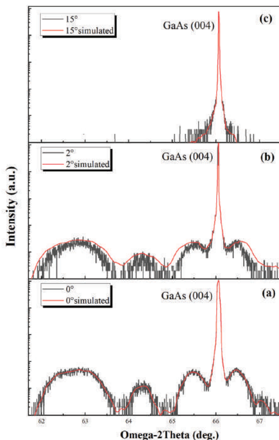
Figure 2. Omega-2 \theta scans around the (004) symmetric XRD patterns of InGaAs/GaAsP QWs grown on substrates with misorientations of (a) 0^\circ , (b) 2^\circ , and (c) 15^\circ .
