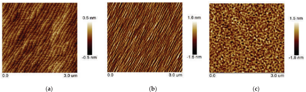
Figure 4. AFM images of InGaAs/GaAsP QWs in a 3 \times 3\text{ }\mu\text{m}^2 scan area with different misoriented substrates: (a) 0^\circ , (b) 2^\circ , and (c) 15^\circ .
