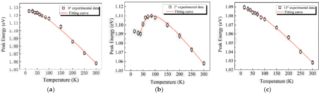
Figure 7. Temperature-dependent peak energies of the InGaAs/GaAsP QWs on (a) 0°, (b) 2°, and (c) 15°-misoriented substrates.
