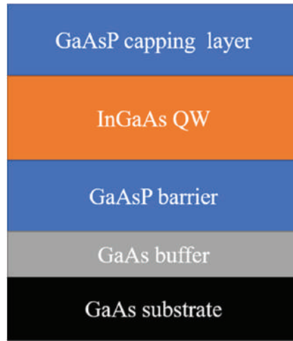
Figure 1. Schematic of the InGaAs/GaAsP quantum well.
