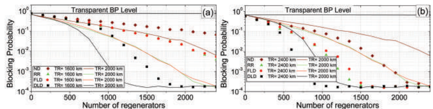
Figure 10. Blocking probability as a function of the total number of regenerators in the CoreNet topology assuming transparent reaches of: (a) T_R = 1600 km; (b) T_R = 2400 km, each compared against the reach of T_R = 2000 km.
