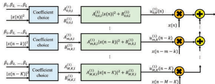
Figure 9. Hardware implementation example using MSA.
