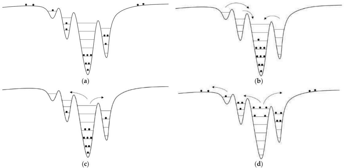
Figure 8. Schematic diagrams illustrating the possible mechanism of the S-shaped temperature-dependent PL peak energy. (a) At the lowest temperature, carriers exist in all possible potential minima. (b) At a slightly higher temperature, carriers relax to the deepest potentials. (c) As the temperature continues to rise, carriers redistribute to higher energies. (d) As the temperature rises very high, most carriers escape from the localization potentials.
