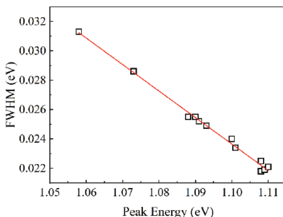
Figure 10. Relationship between photon energy and FWHM for the 2° sample. The red solid line represents the curve fit to the presented data.
