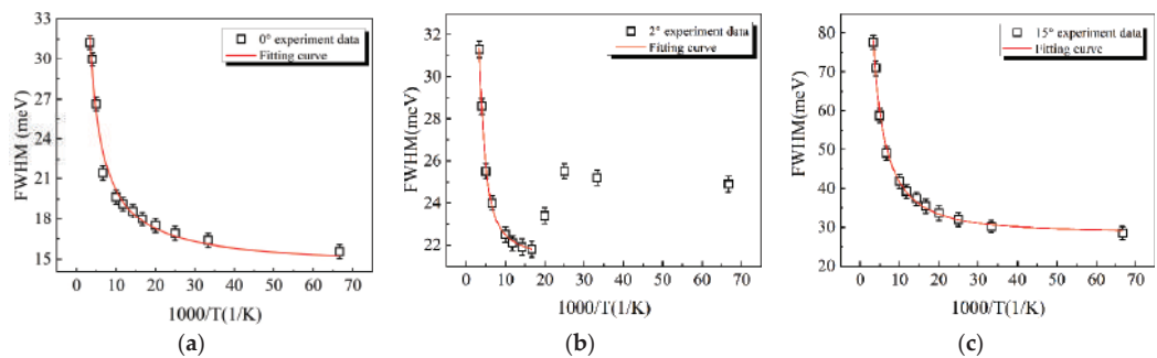
Figure 9. PL full width at half maximum (FWHM) as a function of 1000/T of the InGaAs/GaAsP QWs on substrates misoriented by (a) 0°, (b) 2°, and (c) 15°. The fitting curves of the FWHM data of the PL spectra are predictions based on the exciton–optical phonon coupling model.
