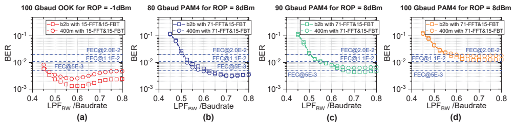
Figure 3. Bit error rate versus \text{LPF}_{\text{BW}}/\text{baud rate} for (a) 100 Gbaud OOK, (b) 80 Gbaud PAM4, (c) 90 Gbaud PAM4, and (d) 100 Gbaud PAM4 signals. We use minus 1 dBm received optical power for OOK and 8 dBm for PAM4 signals.
