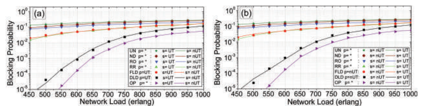
Figure 6. Blocking probability as a function of the total load in CoreNet topology using 1050 regenerators and traffic: (a) uniform and (b) non uniform.
