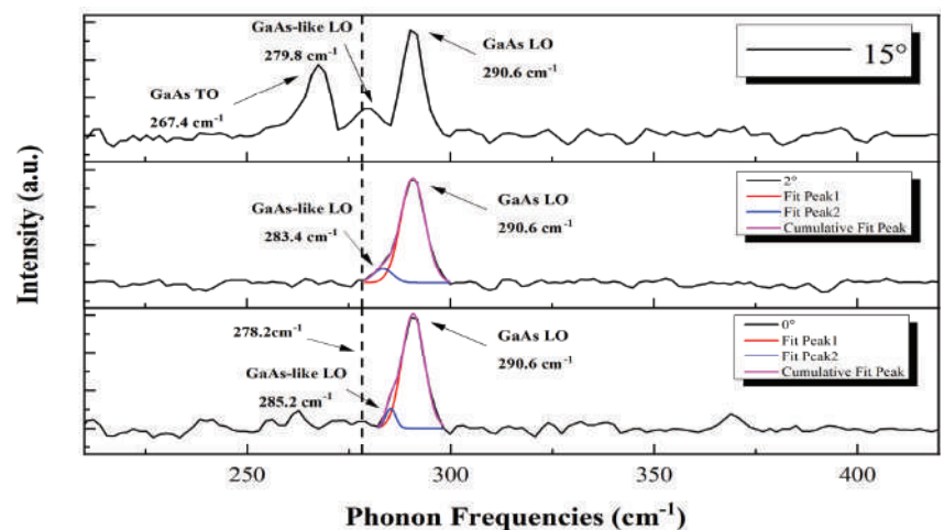
Figure 3. Raman spectra of InGaAs/GaAsP QWs grown on a GaAs (001) substrate with misorientations of 0^\circ , 2^\circ , and 15^\circ using a 488 nm laser.
