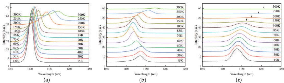
Figure 6. Temperature-dependent of PL spectra for InGaAs/GaAsP QWs on (a) 0^\circ , (b) 2^\circ , and (c) 15^\circ misoriented substrates.
