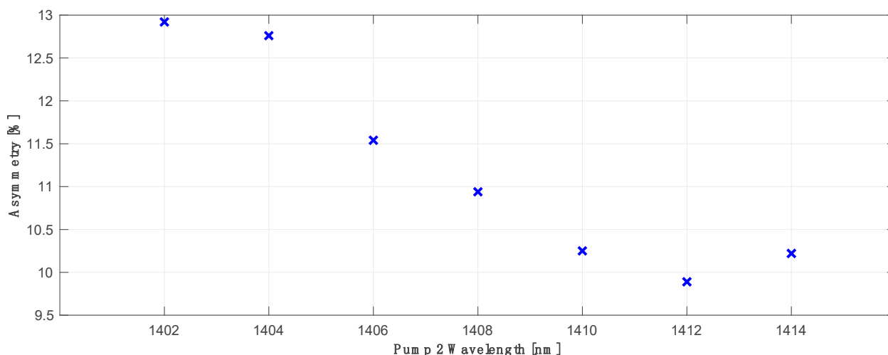
Figure 7. Optimum asymmetry optimization for primary C band pump at 1364 nm and FBG 1458 nm as a function of primary L band pump wavelength for conjugated channels with optimized FBG.
