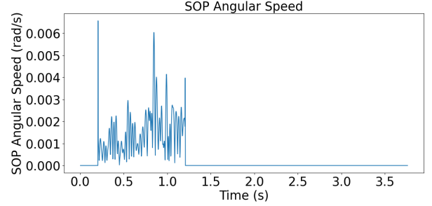
Fig. 7. SOPAS Induced by Additive Strain - Car passage strain over the strain induced by the earthquake
