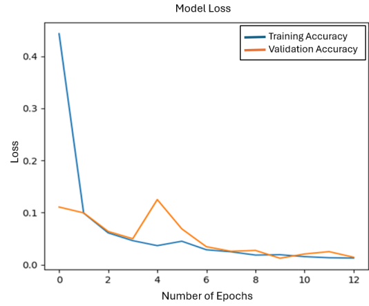
Fig. 9. ML Model Training and Validation Loss
