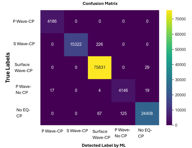
Fig. 10. Confusion Matrix
