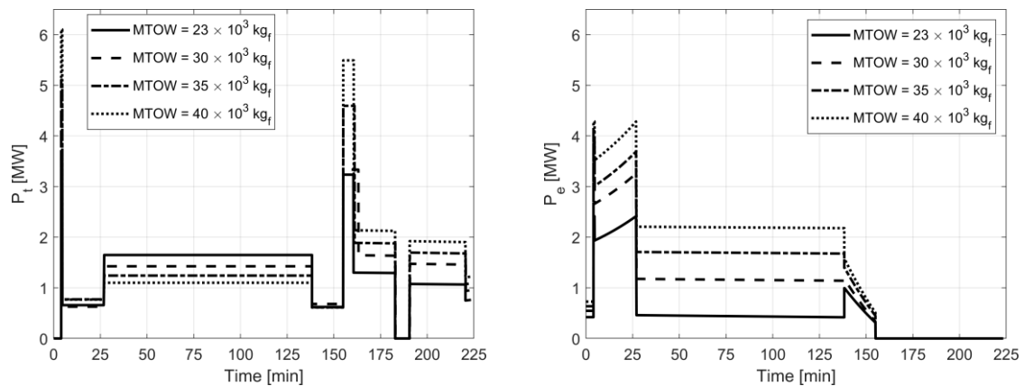
Figure 10 – Mission power profiles varying MTOW: thermal(left) and electric (right).
