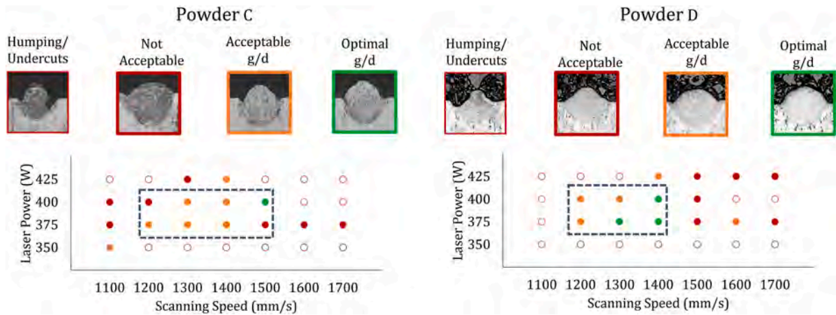
Fig. 15. Process maps for powders C and D. The identified process window is highlighted by the contour.
