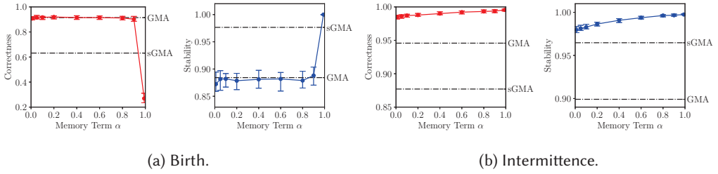
Fig. 8. Impact of memory term \alpha on correctness and stability of \alpha GMA for birth (morphing) and intermittence (noise) transformations.
