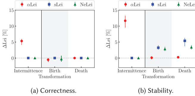
Fig. 5. Leiden-based algorithms. Median gain and bootstrapped 99% confidence interval in Correctness and Stability for the three transformations with larger differences. The vertical solid line distinguishes between noise and morphing scenarios.
