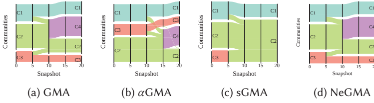
Fig. 6. Example of the dynamic evolution of the graph with instantaneous birth transformation at time 10, showing the community assignment (GMA-based algorithms).
