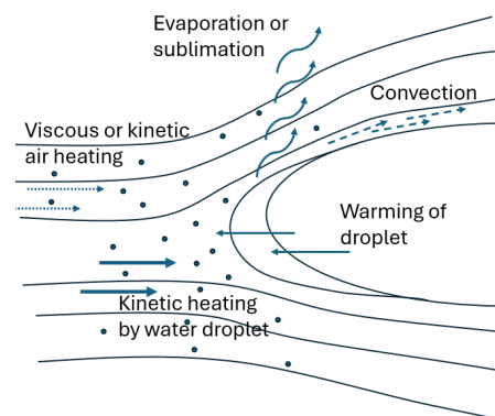
Figure 19. Thermal contributions experienced by the wing profile [11].
