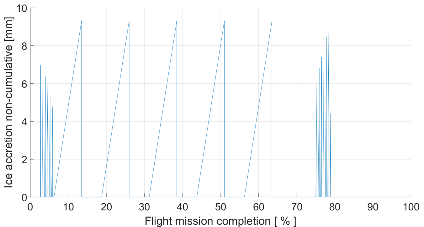
Figure 17. Graph of ice accretion on wings (non-cumulative) throughout the flight mission.
