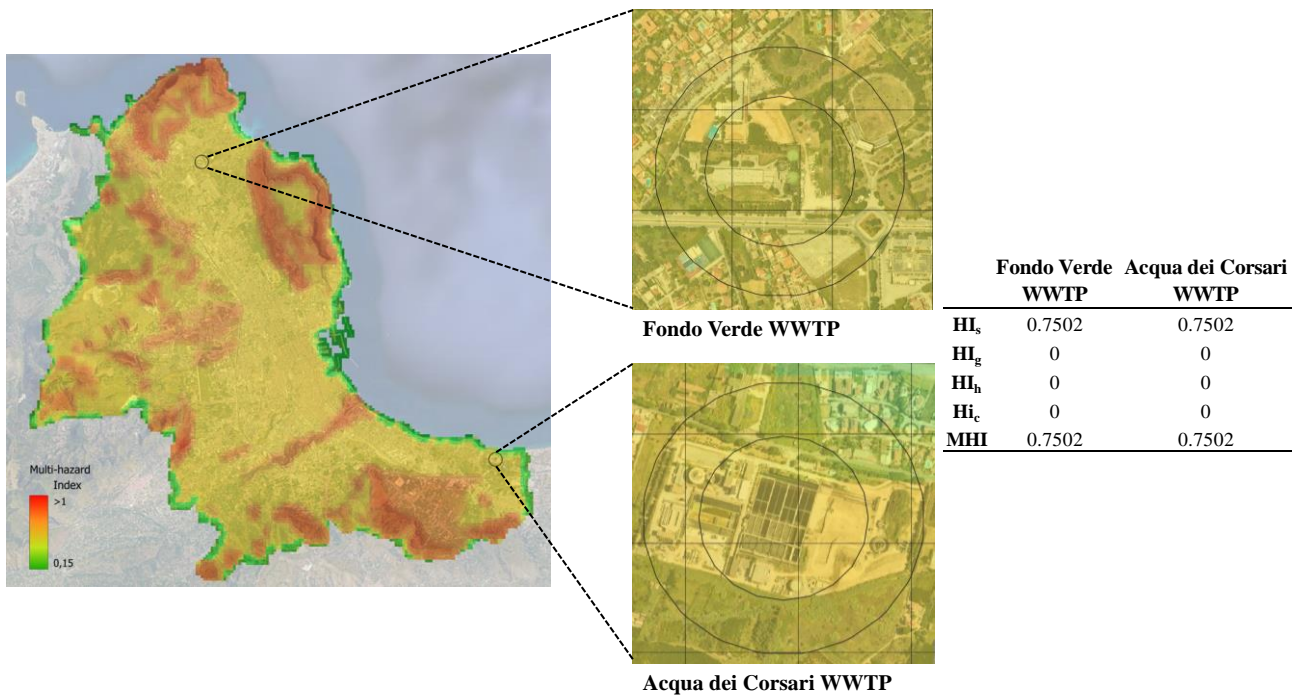
Figure 4. Multi-hazard index mapping of the municipality of Palermo with a focus on the two WWTPs.
