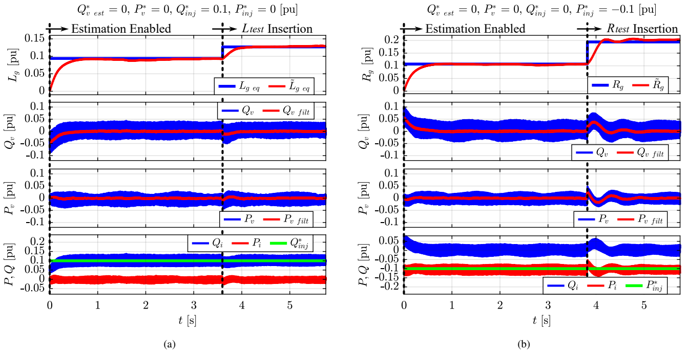
Fig. 8. Results of Test 2: grid inductance (a) and resistance (b) estimation by respectively setting the external references Q_{inj}^* = 0.1 and P_{inj}^* = -0.1 pu. Meanwhile, the VSM operates at null power ( Q_{v,est}^* = P_v^* = 0 ). From top to bottom: measured L_{g\ eq} - R_{g\ eq} and estimated \tilde{L}_{g\ eq} - \tilde{R}_{g\ eq} values of grid inductance and resistance; unfiltered Q_v and filtered Q_{v\ filt} virtual reactive power; unfiltered P_v and filtered P_{v\ filt} virtual active power; inverter output power Q_i - P_i and injected power references Q_{inj}^* - P_{inj}^* .
