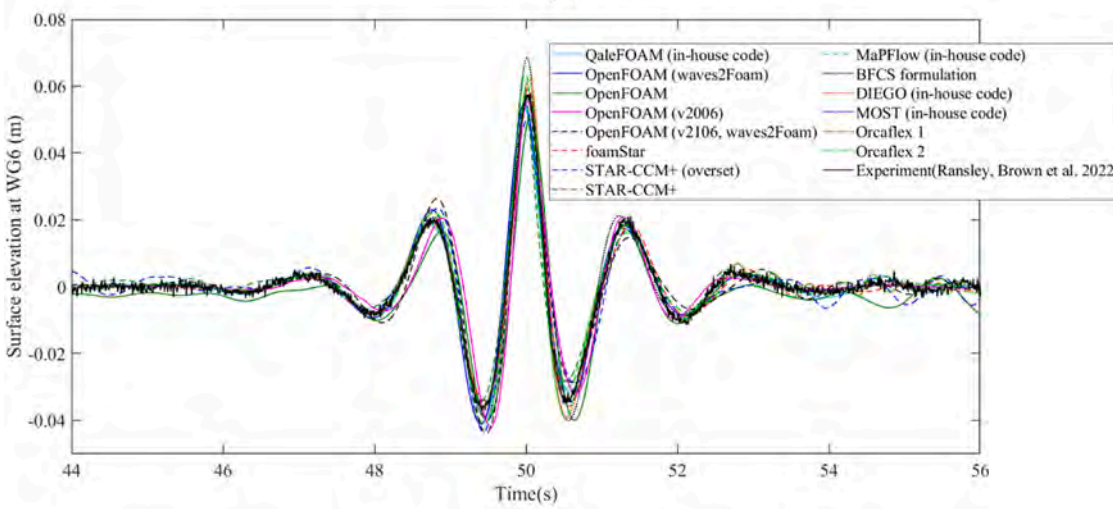
Fig. 9. Surface elevation measured at WGs 4, 6 and 8 from an empty tank test for focused wave cases: (a), (c) and (e) operational case and (b), (d) and (f) extreme case.
