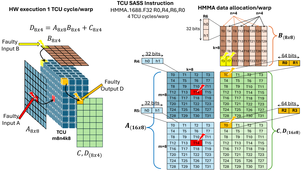
Fig. 8. Modeling the effect of permanent faults on the Ampere's TCU while executing the HMMA. 1688 instruction. According to the A100 Ampere architecture, the TCU hardware performs one 8 \times 4 \times 8 Matrix Multiplication in one clock cycle per warp (i.e., 32 threads) [13]. In addition, the HMMA. 1688 instruction spends four clock cycles to compute a Matrix Multiplication (MM) of shape 16 \times 8 \times 8 [13]. Therefore, one fault in the TCU hardware can be modeled by corrupting four values in the input and output matrices of the executed instruction (i.e., A, B, C, or D).
