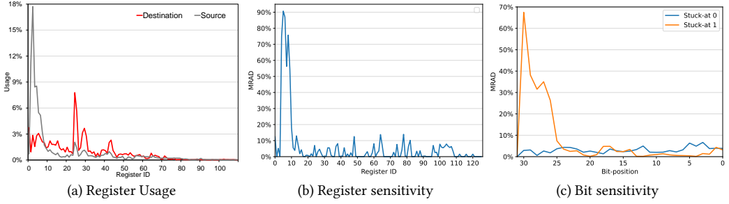
Fig. 9. Usage of GPU's Registers and Sensitivity of GPU's Registers to Permanent Faults.
