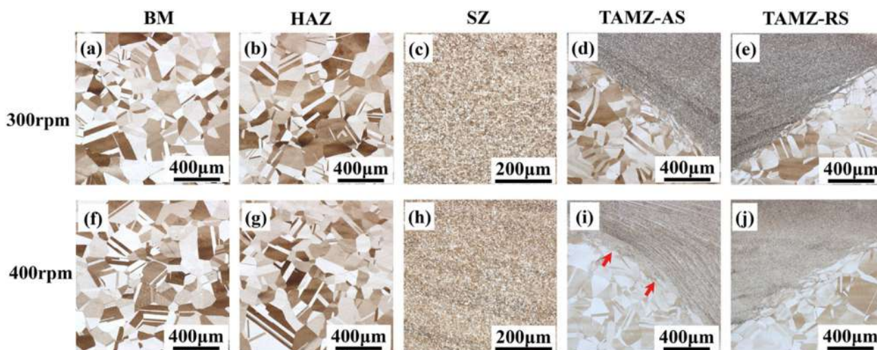
Figure 10. Butt FSW of 2.4 mm thick S32654. Optical images of various microstructural zones: BM (a,f), HAZ (b,g), SZ (c,h), TMAZ-AS (d,i) and TMAZ-RS (e,j) of 300 and 400 rpm, respectively ( v 100 mm/min) [111]. Red arrows highlight the TMAZ region.
