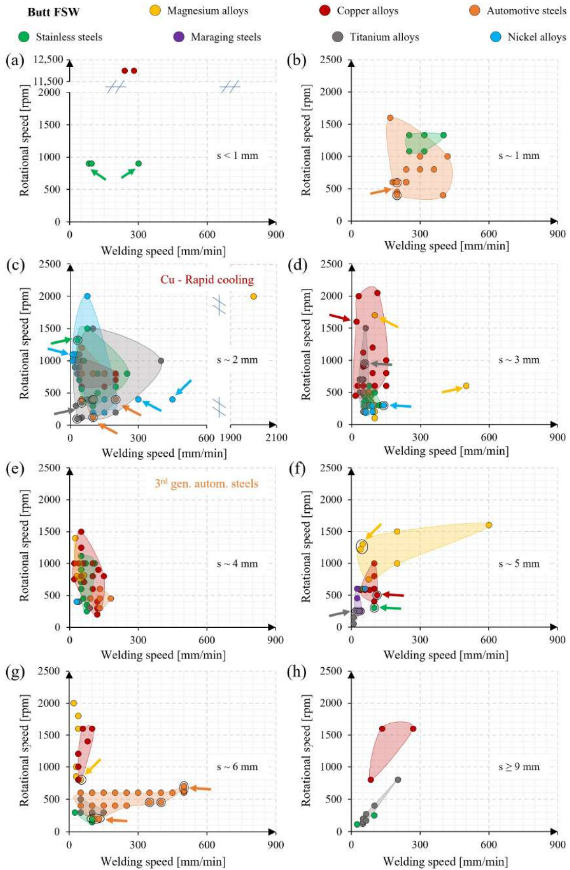
Figure 16. Rotational vs. welding speed for butt FSW of the investigated alloys. Images are grouped based on sheet thickness: (a) <1 mm (i.e., 0.5–0.6 mm), (b) \sim 1 mm (i.e., 1.0–1.6 mm), (c) \sim 2 mm (i.e., 1.8–2.5 mm), (d) \sim 3 mm (i.e., 2.9–3.5 mm), (e) \sim 4 mm (i.e., 3.8–4.0 mm), (f) \sim 5 mm (i.e., 4.8–5.5 mm), (g) \sim 6 mm (i.e., 6.0–6.5 mm), (h) \geq 9 mm (i.e., 9.0–12.7 mm). Arrows highlight some specific points that are detailed in the main text.
