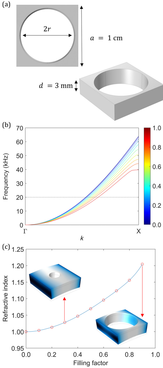
FIG. 2. (a) Representation of the unit cell: the filling factor is a parameter equal to 2r/a , which is used to quantify the grading. (b) Redshift of the A_0 mode with increasing filling factor: eigenfrequency simulations with Bloch-Floquet conditions were run on unit cells with filling factors ranging from 0.1 to 0.9. (c) Bijective relation between the filling factor and the refractive index n = k/k_0 .
