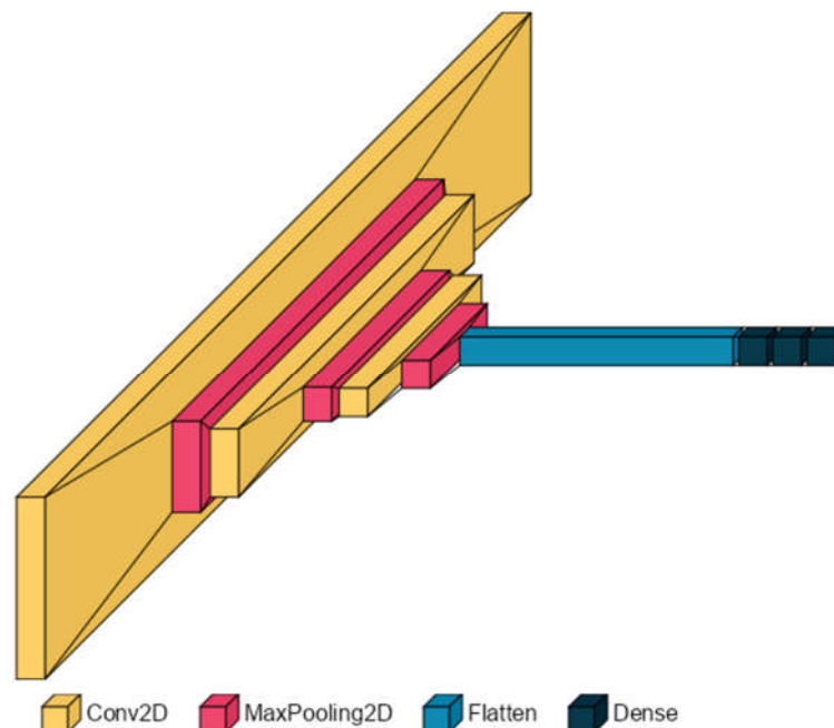
Figure 5. CNN Architecture.
