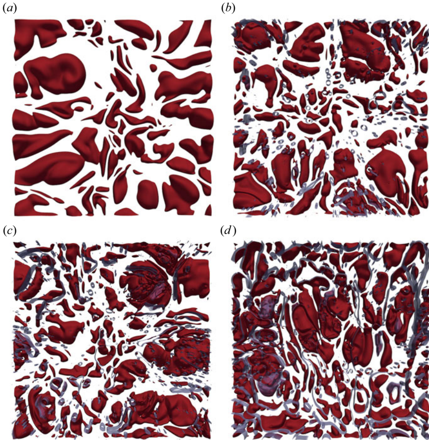
Figure 6. A top view of the instantaneous temperature isosurfaces (red colour) in \tilde{x}-\tilde{y} plane inside the hot-plate boundary layers at \hat{\theta} = 0.3 and for various dispersed-droplet volume fractions of (a) \Phi = 0 , (b) \Phi = 0.2 , (c) \Phi = 0.4 and (d) \Phi = 0.5 . Dispersed droplets are shown with a grey colour.
