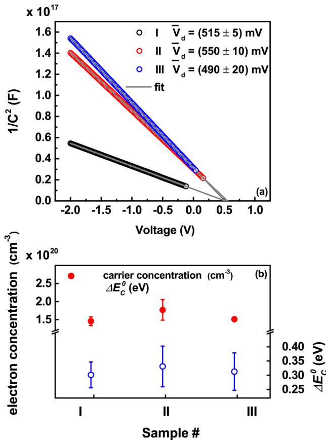
FIG. 9. (a) Plot of 1/C^2 measured at 200 kHz vs the applied voltage in the case of three selected test structures with the extracted \bar{V}_d (average between the five different probing frequencies used) reported in the figure as well. (b) n and the extracted \Delta E_C^0 s. In both figures, I, II, and III indicate the series with the first TMA pulse introduced after a total number of DEZ+DI and MCp2Mg+DI pulses equal to 24, 96, and 384, respectively. The Mg content in the samples series shown here varied between (9.1 \pm 0.3) and (9.9 \pm 0.3) at. %.
