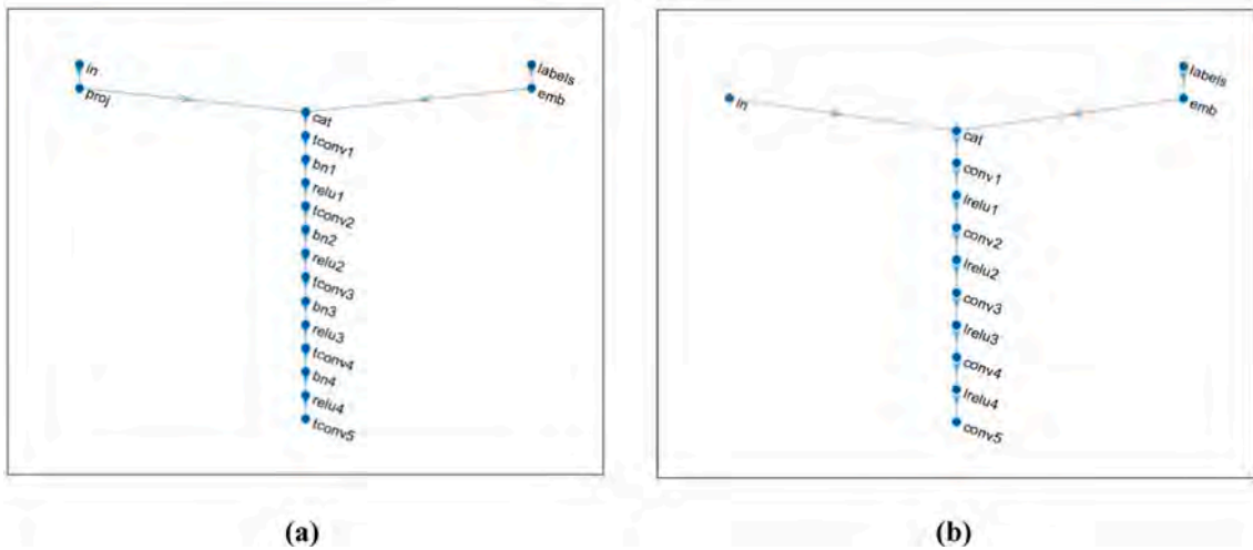
Fig. 2. Architectures of G (a) and D (b). in: input layer; proj: project and reshape layer; labels: label layer; emb: embedding and reshape layer; cat: concatenation layer; tconv: transposed convolutional 2D layer; bn: batch normalization layer; relu: ReLU layer; lrelu: leaky ReLU layer.
