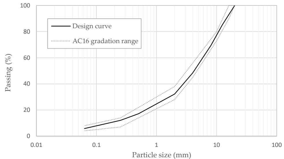
Figure 2. Gradation limits and target gradation curve of AC mixtures.
