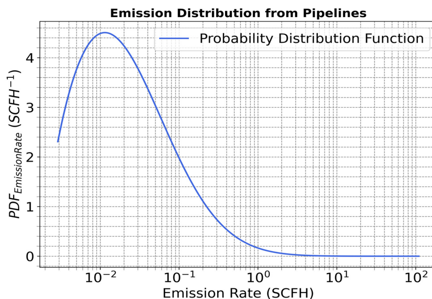
Figure 3. Emission distribution for mainlines and service lines resulting from a lognormal fit to the sample. The emission distribution is skewed, meaning that a small portion of emission rates is significantly higher than the mode.
