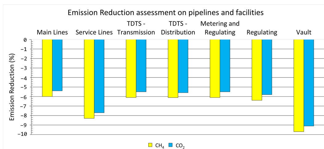
Figure 9. Emission reduction assessment consequential to hydrogen blending into the distribution system and comparison of CH 4 emission reduction versus equivalent CO 2 emission reduction to account for the global warming potential of H 2 leakage.
