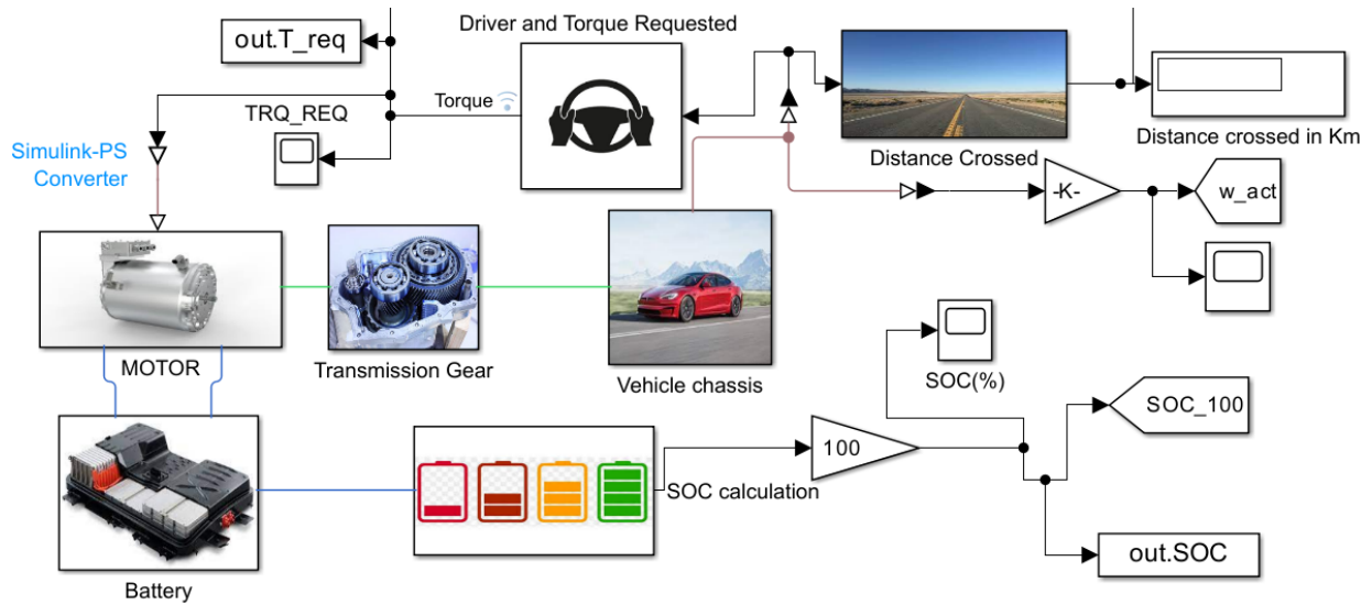
Fig. 1: Full BEV Simulink model.
