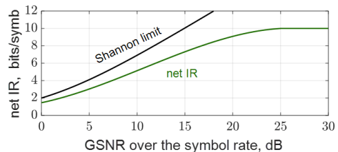
Fig. 5: Transponder net user information rate vs. GSNR.
