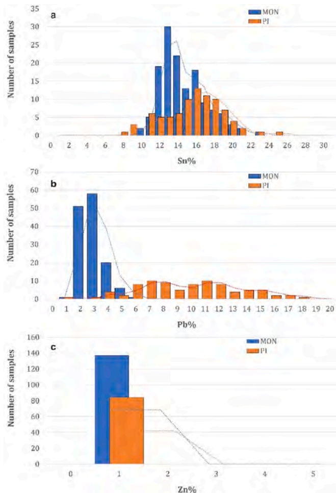
Fig. 12. Frequency distribution of the main alloying elements from the XRF analyses of the panels of two doors analysed (MON=Monreale; PI=Pisa): a) Sn; b) Pb; c) Zn.
