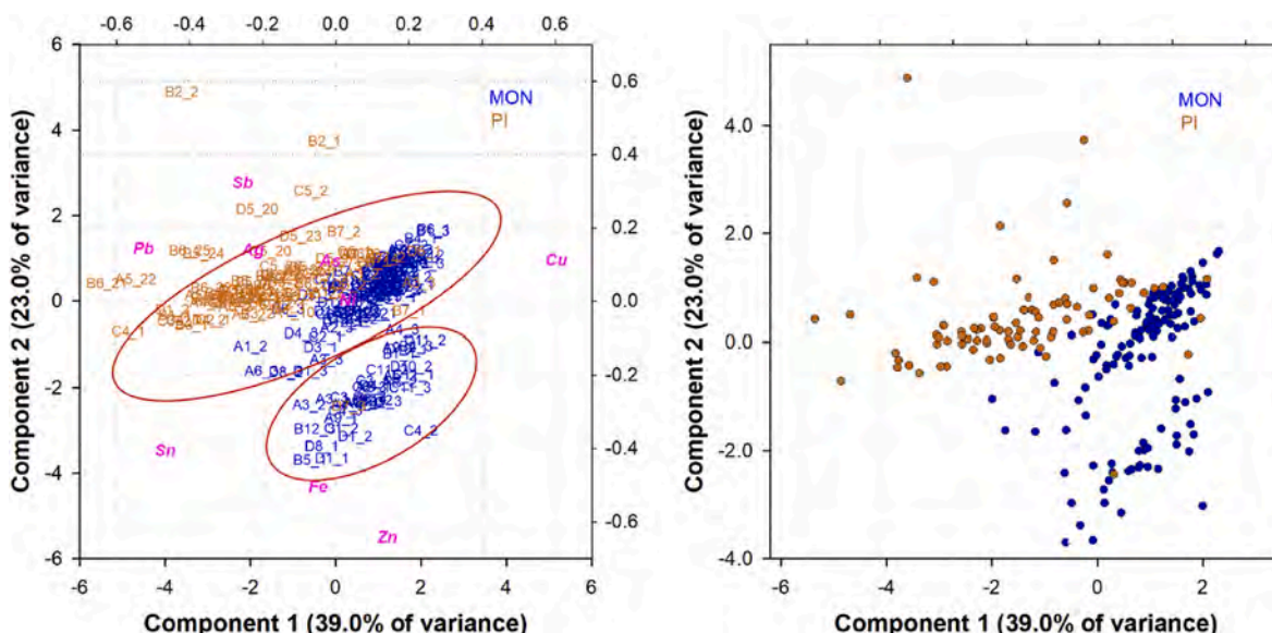
Fig. 11. PCA computation (PC1 vs PC2, total explained variance of 62.0%) on the panels of the doors: MON=Monreale; PI=Pisa. a) biplot; b) score plot.
