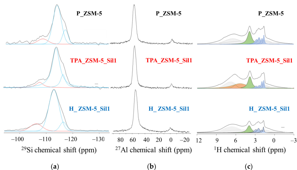
Figure 3. (a) ^{29}\text{Si} NMR spectra, blue lines correspond to Q4 sites, red lines correspond to Q 3 sites, (b) ^{27}\text{Al} NMR spectra, (c) ^1\text{H} NMR spectra, blue lines correspond to isolated and weakly H-bonded silanols, green lines correspond to isolated BAS while orange lines correspond to strongly H-bonded silanols and BAS, grey lines are due to 1.9 mm rotor caps. All samples were pretreated at 623 K under high vacuum ( 10^{-6}\text{ kPa} ) and the rotors were closed in a glove box under Ar before the acquisition of the spectra. The intensity of the rotor signal (slightly shifting due to differences in magnetic susceptibilities of the samples) was kept constant during the fitting procedure for all samples as in reference [3].
