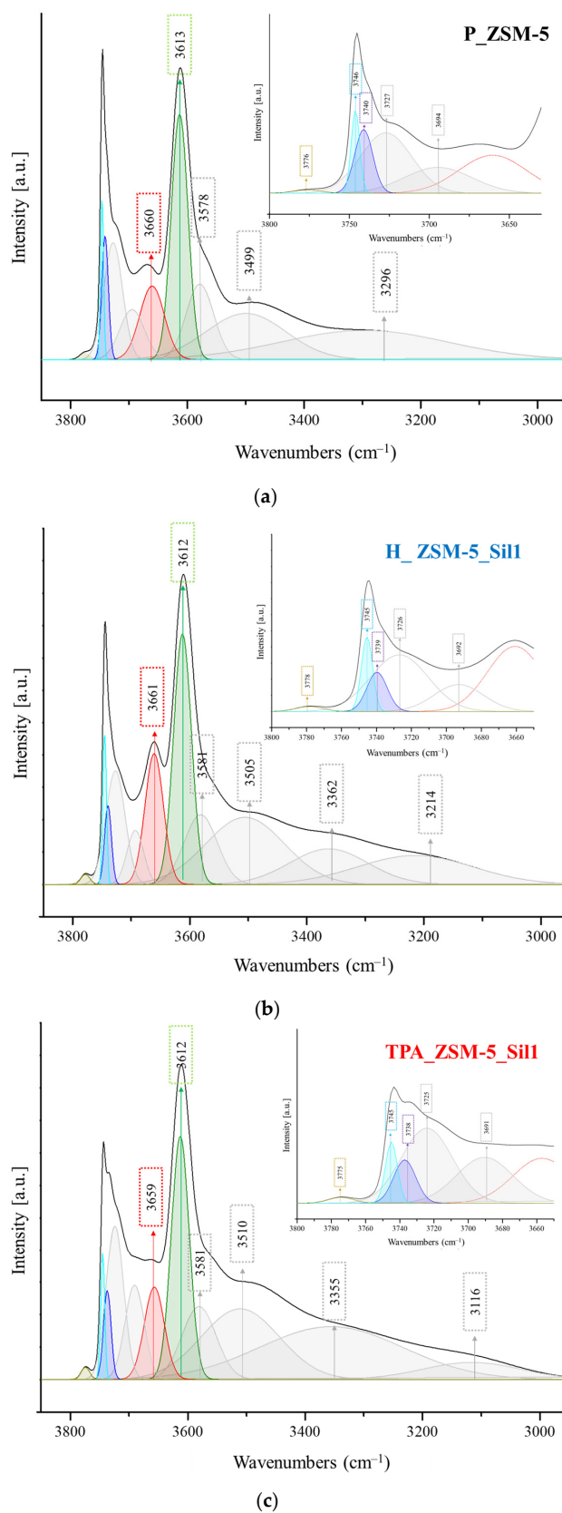
Figure 2. FTIR spectra of the activated P_ZSM-5 (a), H_ZSM-5_Sil1 (b), and TPA_ZSM-5_Sil1 (c) samples in the region 3900–3200 cm -1 with the respective deconvolution curves. Inset: Spectra presented in the range of 3600–3800 cm -1 .
