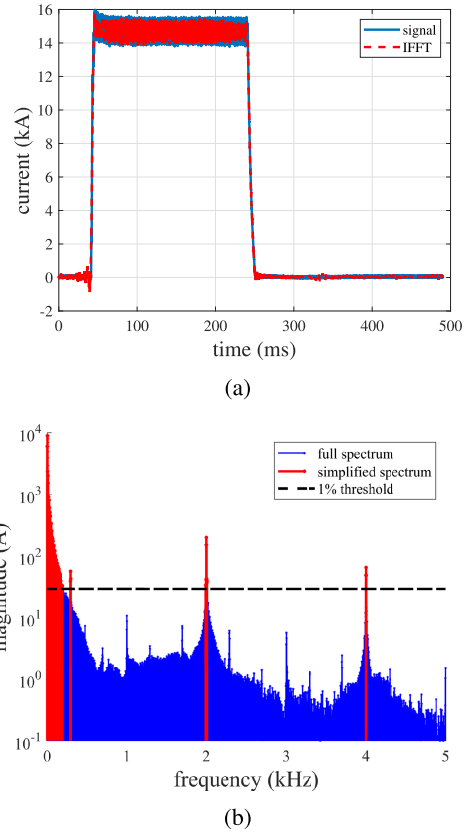
FIGURE 6. Real welding current pulse measured at Polito (in blue) with the simplified pulse considered in our simulation (in red) (a), original and simplified spectrum of the measured current pulse with the black line at 1% of the fundamental (b).
