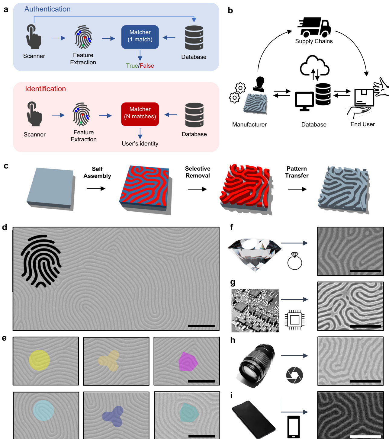
Fig. 1 | Artificial fingerprints as physical unclonable functions for authentication and identification. a Graphical workflow of authentication and identification processes through fingerprints. b Product's identification/authentication through artificial fingerprints. The artificial fingerprint can be physically transferred on the surface of the product by the manufacturer right after its production and subsequently registered and stored in the database. The product is then delivered to the buyer and the identification/authentication of the product can be performed directly by the end user by comparing the artificial fingerprint with fingerprints stored in the database. c Schematics of fabrication procedure by BCP self-assembly and pattern transfer for the realization of artificial nano-fingerprints. d SEM images
