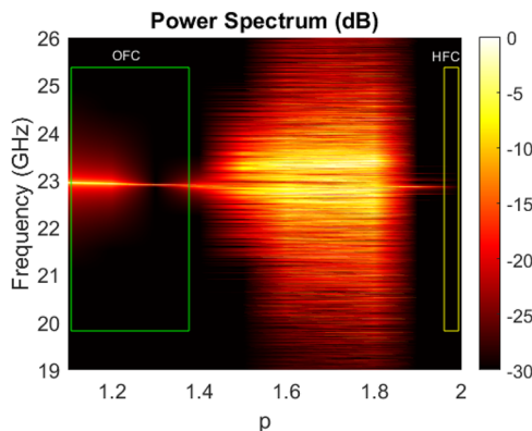
FIG. 4. First beatnote observed in the power spectrum while varying the pump parameter p in the FP configuration, with \Gamma = 0.03 , \alpha = 1.3 , and other parameters as specified in Fig. 2. We highlight in green the region of dense OFCs and in yellow the region of HFCs.
