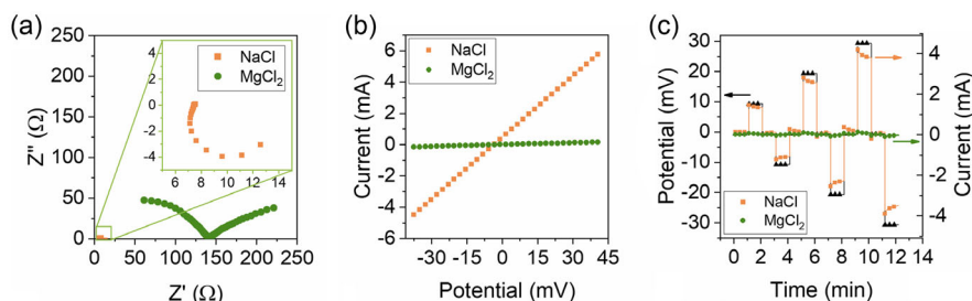
Figure 5. Ionic resistance measurements of GO-KOH after being immersed for 1 h in NaCl (in orange) and \text{MgCl}_2 (in green) 0.5 M a) EIS b) LSV, and c) chronoamperometry, with the applied potential (in black) and the measured current for NaCl (in orange) and \text{MgCl}_2 (in green).
