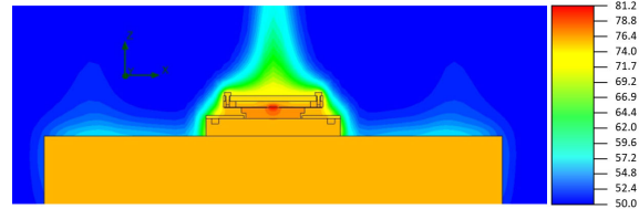
Fig. 11. Thermal simulation of the carrier. (a) Thermal stack-up. (b) Results at 75^\circ\text{C} Peltier and 50^\circ\text{C} ambient temperature.
