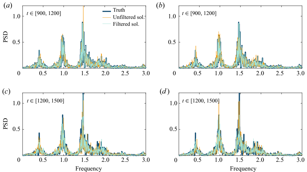
Figure 20. Power spectral density (PSD) during (a,b) and after (c,d) assimilation of the true pressure oscillations (dark blue), unfiltered solution (orange) and filtered solution (light blue), during state estimation in a chaotic regime ( \beta = 7.0 ). (a,c) Assimilation of acoustic modes. (b,d) Assimilation of pressure from microphones. Here, m = 100 , \sigma_{mic} = 0.01 , \sigma_{frac} = 0.25 and \Delta t_{analysis} = 0.5 .
