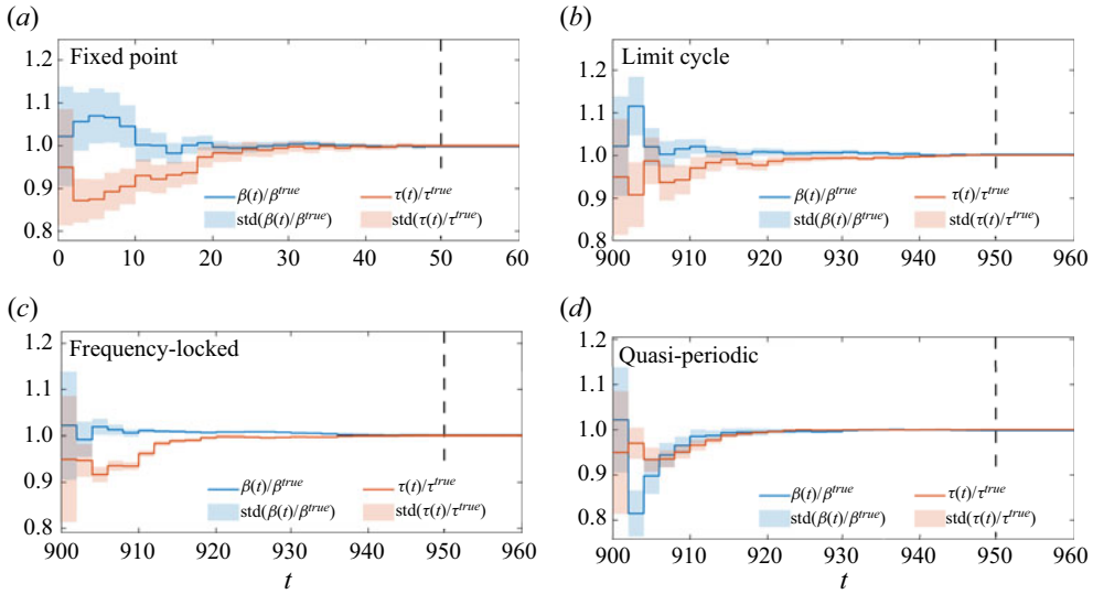
Figure 10. Real-time learning of the parameters and the state. Assimilation of acoustic modes for combined state and parameter estimation of non-chaotic regimes: (a) transient towards a fixed point ( \beta^{true} = 0.2 ); (b) limit cycle ( \beta^{true} = 0.4 ); (c) frequency-locked solution ( \beta^{true} = 7.7 ); and (d) quasi-periodic solution ( \beta^{true} = 3.6 ). The dashed vertical line indicates when data assimilation ends. Here, \tau^{true} = 0.2 , m = 10 , \sigma_{frac} = 0.25 and \Delta t_{analysis} = 2 .
