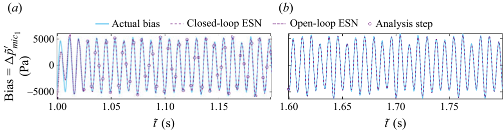
Figure 24. Real-time learning of the model bias and unbiased state. Comparison of the actual bias and the estimated model bias from the ESN during state estimation. (a) Open-loop initialisation and sequential closed loops re-initialised at analysis steps. (b) Echo state network's closed-loop forecast after data assimilation ends.
