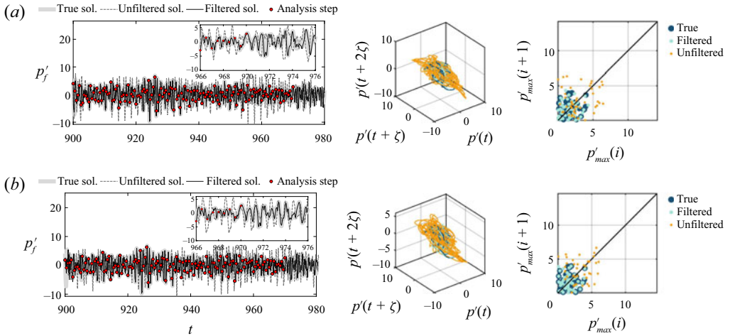
Figure 19. Real-time learning of the state. Assimilation of (a) acoustic modes and (b) pressure from microphones for state estimation of a chaotic regime ( \beta = 7.0 ). Left-hand plots: true pressure oscillations at the flame location (light grey), unfiltered solution (dashed dark grey) and filtered solution (black). The analysis time steps are indicated with red circles. Centre and right-hand plots: phase portrait and first return map of the true (dark blue), filtered (light blue) and unfiltered (orange) solutions. Here, m = 100 , \sigma_{mic} = 0.01 , \sigma_{frac} = 0.25 and \Delta t_{analysis} = 0.5 .
