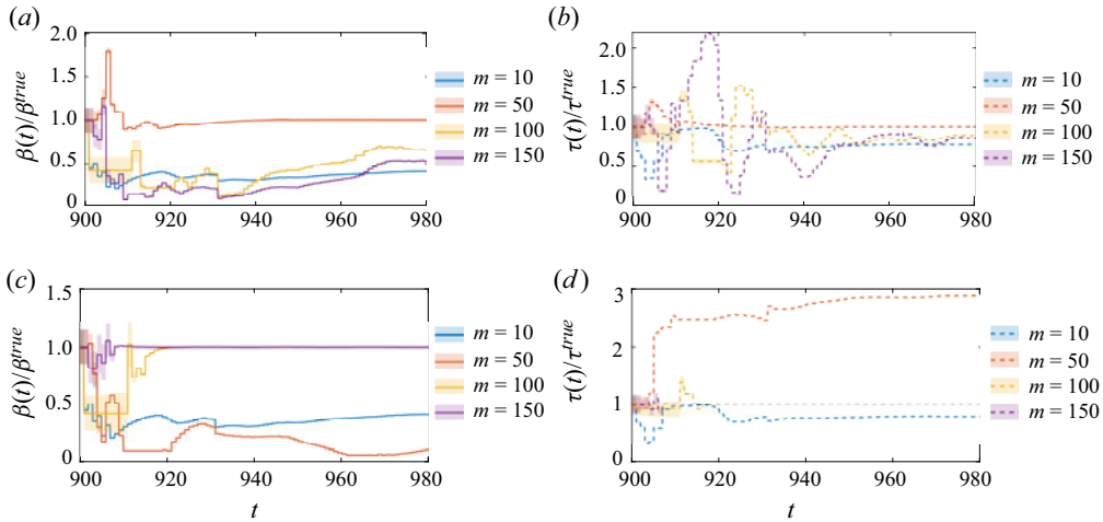
Figure 15. Real-time learning of the parameters. Assimilation of acoustic pressure from microphones for combined state and parameter estimation of a quasi-periodic solution: (a,c) normalised \beta ; (b,d) normalised \tau . Effect of ensemble size is shown without inflation (a,b), and with inflation using \rho = 1.02 (c,d). Here, N_{mic} = 15 , \beta^{true} = 3.6 , \tau^{true} = 0.2 , \Delta t_{analysis} = 1 and \sigma_{mic} = 0.01 . The shaded areas show the standard deviation, which becomes smaller as more data are assimilated.
