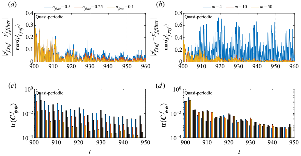
Figure 9. Assimilation of acoustic modes for state estimation of a quasi-periodic regime – performance metrics. (a,c) Effect of the standard deviation with m = 10 . (b,d) Effect of the ensemble size with modes measurement uncertainty \sigma_{frac} = 0.25 . The error evolution is shown with the relative difference between the filtered solutions and truth (a,b) and the trace of the ensemble covariance (c,d). The dashed vertical line indicates when data assimilation ends. Here, \beta = 3.6 and \Delta t_{analysis} = 2 .
