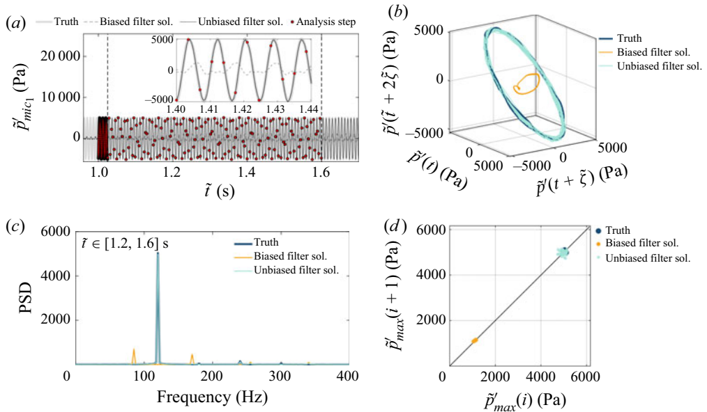
Figure 23. Real-time learning of the model bias and unbiased state. (a) True pressure oscillations at \tilde{x}/\tilde{L}_0 = 0.18 (light grey), biased filtered solution (dashed dark grey) and unbiased filtered solution (black). The analysis time steps are indicated with red circles; the vertical dashed lines show the assimilation window. (b) Phase portrait, (c) power spectral density (PSD), and (d) first return map of the true pressure oscillations (dark blue), biased filtered solution (orange) and unbiased filtered solution (light blue).
