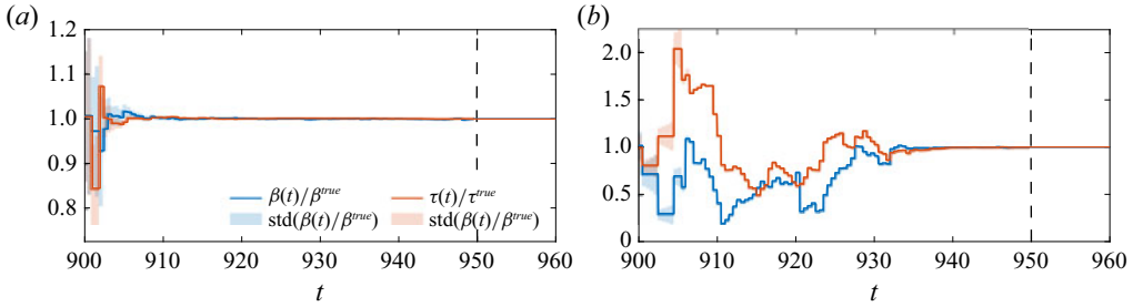
Figure 21. Real-time learning of the parameters. Assimilation of (a) acoustic modes and (b) pressure from microphones for combined state and parameter estimation of a chaotic regime. Time evolution of the parameters and their standard deviation. Chaotic solution ( \beta = 7.0 ). The dashed vertical line indicates when data assimilation ends. Here, m = 300 , \rho = 1.2 , \sigma_{mic} = 0.01 , \Delta t_{analysis} = 0.5 and N_{mic} = 6 .
