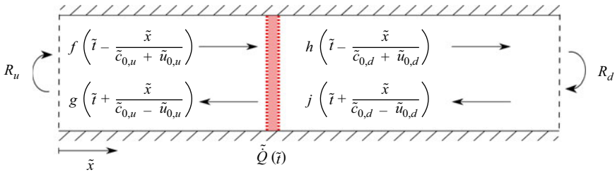
Figure 5. Schematic of the acoustic waves travelling upstream and downstream of a flame in an open-ended tube.
