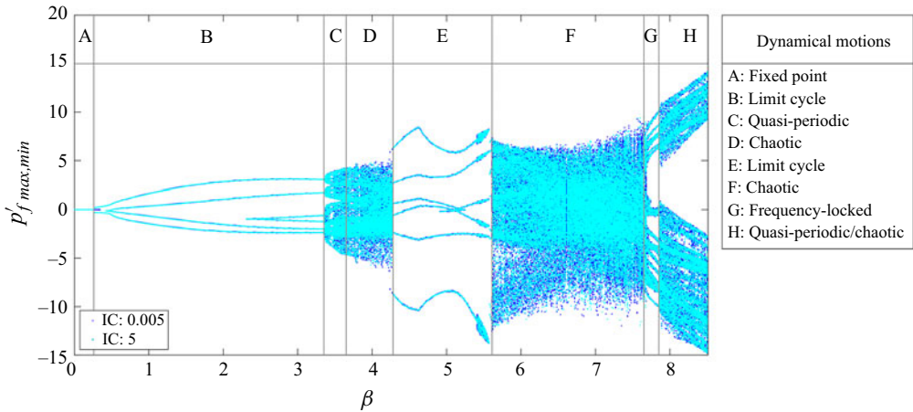
Figure 7. One-dimensional bifurcation diagram. Maxima and minima of the pressure oscillations at the flame location versus the heat-source strength. The solutions obtained for small/large initial conditions (IC) are shown in a dark/light blue. This diagram identifies different nonlinear behaviours, which have implications for data assimilation.
