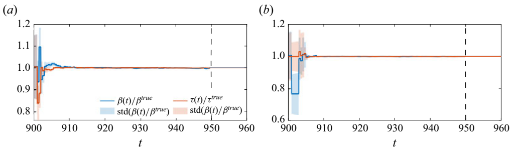
Figure 22. Real-time learning of the parameters. Assimilation of (a) acoustic modes and (b) pressure from microphones for combined state and parameter estimation of a chaotic regime. Time evolution of the parameters and their standard deviation. Chaotic solution ( \beta = 7.0 ). The dashed vertical line indicates when data assimilation ends. Here, m = 300 , \rho = 1.02 , \sigma_{mic} = 0.01 , \Delta t_{analysis} = 0.5 and N_{mic} = 15 .
