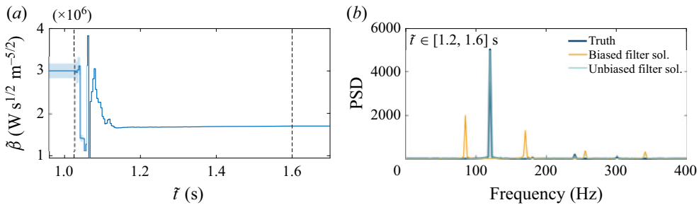
Figure 25. Real-time learning of the model bias, unbiased state and parameters. (a) Time evolution of the parameter \tilde{\beta} with the standard deviation. (b) Power spectral density (PSD) of the pressure oscillations at \tilde{x}/\tilde{L}_0 = 0.18 of the true pressure oscillations (dark blue), biased filtered solution (orange) and unbiased filtered solution (light blue). The vertical dashed lines show the assimilation window.
