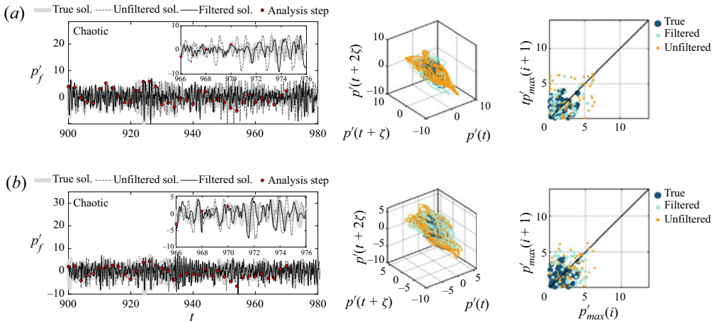
Figure 16. Real-time learning of the state. Assimilation of (a) acoustic modes and (b) pressure from microphones for state estimation of a chaotic regime ( \beta = 7.0 ). Left-hand plots: true pressure oscillations at the flame location (light grey), unfiltered solution (dashed dark grey) and filtered solution (black). The analysis time steps are indicated with red circles. Centre and right-hand plots: phase portrait and first return map of the true (dark blue), filtered (light blue) and unfiltered (orange) solutions. Here, m = 10 , \sigma_{mic} = 0.01 , \sigma_{frac} = 0.25 and \Delta t_{analysis} = 2 .
