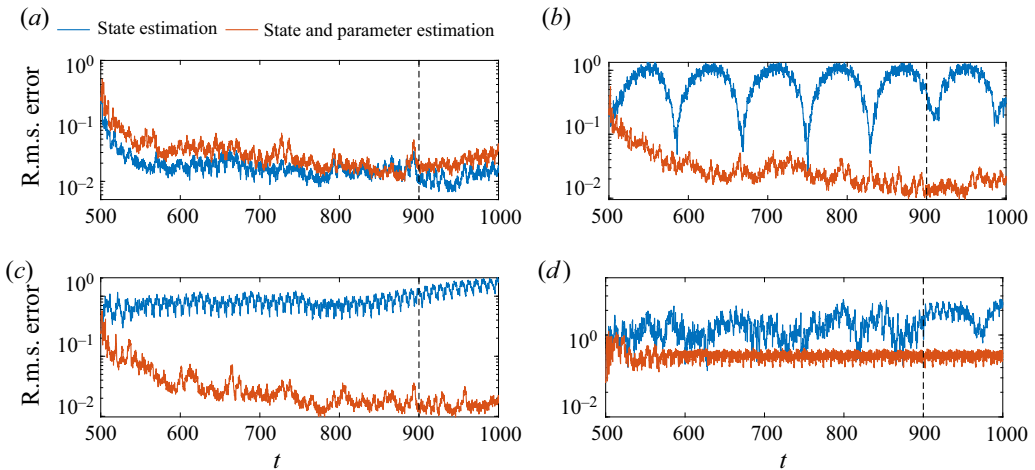
Figure 11. Assimilation of acoustic modes of a quasi-periodic regime. Performance of state estimation (blue) versus combined state and parameter estimation (orange) in a quasi-periodic regime. Initial conditions \beta = c \beta^{true} and \tau = c \tau^{true} , with (a) c = 1 , (b) c = 1.05 , (c) c = 1.25 , (d) c = 1.5 ; and \beta^{true} = 3.6 , \tau^{true} = 0.2 . The dashed vertical line indicates when data assimilation ends.
