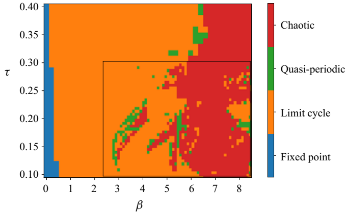
Figure 6. Two-dimensional bifurcation diagram. Classification of the attractor of the thermoacoustic system. The area enclosed by the black rectangle corresponds to a refined grid. The coarse and fine sweeps are performed with resolutions (\Delta\beta, \Delta\tau) = (0.2, 0.01) and (\Delta\beta, \Delta\tau) = (0.1, 0.005) , respectively.
