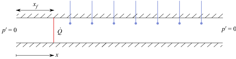
Figure 1. Schematic of an open-ended duct with a heat source (also known as the Rijke tube). The heat released by the compact heat source is indicated by the vertical dotted line. The blue vertical lines indicate microphones located equidistantly.
