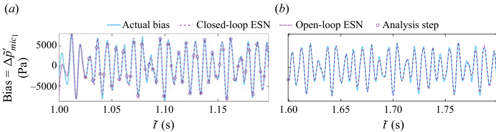
Figure 26. Real-time learning of the model bias, unbiased state and parameters. Comparison of the actual bias and the estimated model bias from the ESN during state and parameter estimation. (a) Open-loop initialisation and sequential closed loops re-initialised at analysis steps. (b) Echo state network's closed-loop forecast after data assimilation ends.
