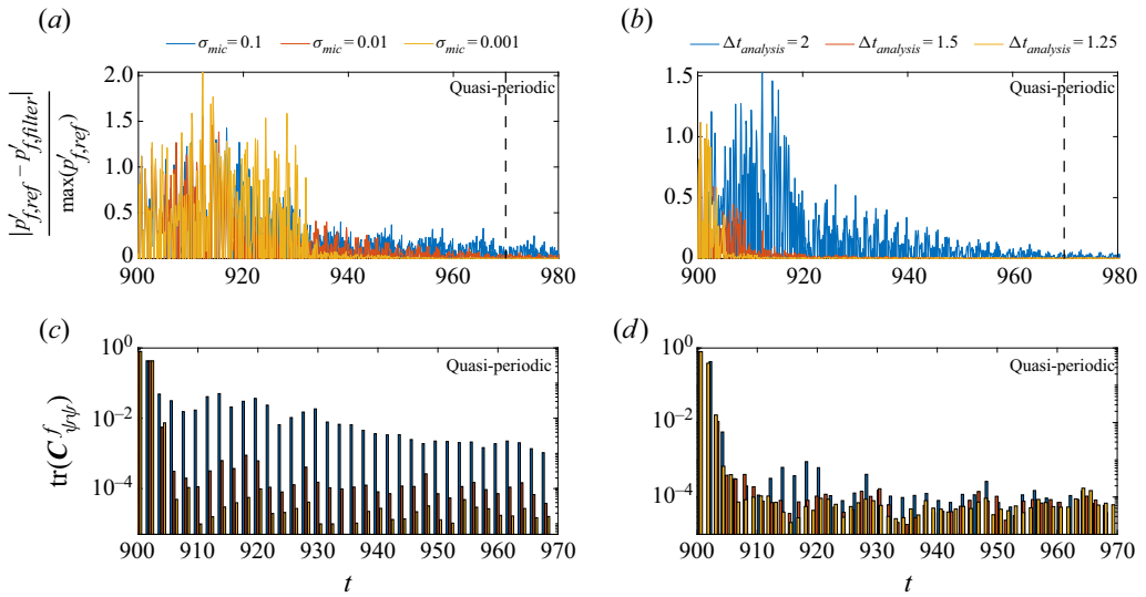
Figure 13. Assimilation of pressure from microphones for state estimation of a quasi-periodic regime. Performance metrics. (a,c) Effect of the microphones’ standard deviation with \Delta t_{analysis} = 2 . (b,d) Effect of the assimilation frequency with \sigma_{mic} = 0.01 . The error evolution is shown with the relative difference between the true and filtered solutions (a,b) and the trace of the ensemble covariance (c,d). The dashed vertical line indicates when data assimilation ends. Here, \beta = 3.6 and m = 10 .
