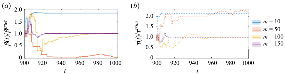
Figure 14. Real-time learning of the parameters. Assimilation of acoustic pressure from microphones for combined state and parameter estimation of a quasi-periodic solution: (a) normalised \beta ; (b) normalised \tau . Here, N_{mic} = 6 , \beta^{true} = 3.6 , \tau^{true} = 0.2 , \Delta t_{analysis} = 1.5 and \sigma_{mic} = 0.01 . The shaded areas show the standard deviation, which becomes smaller as more data are assimilated.
