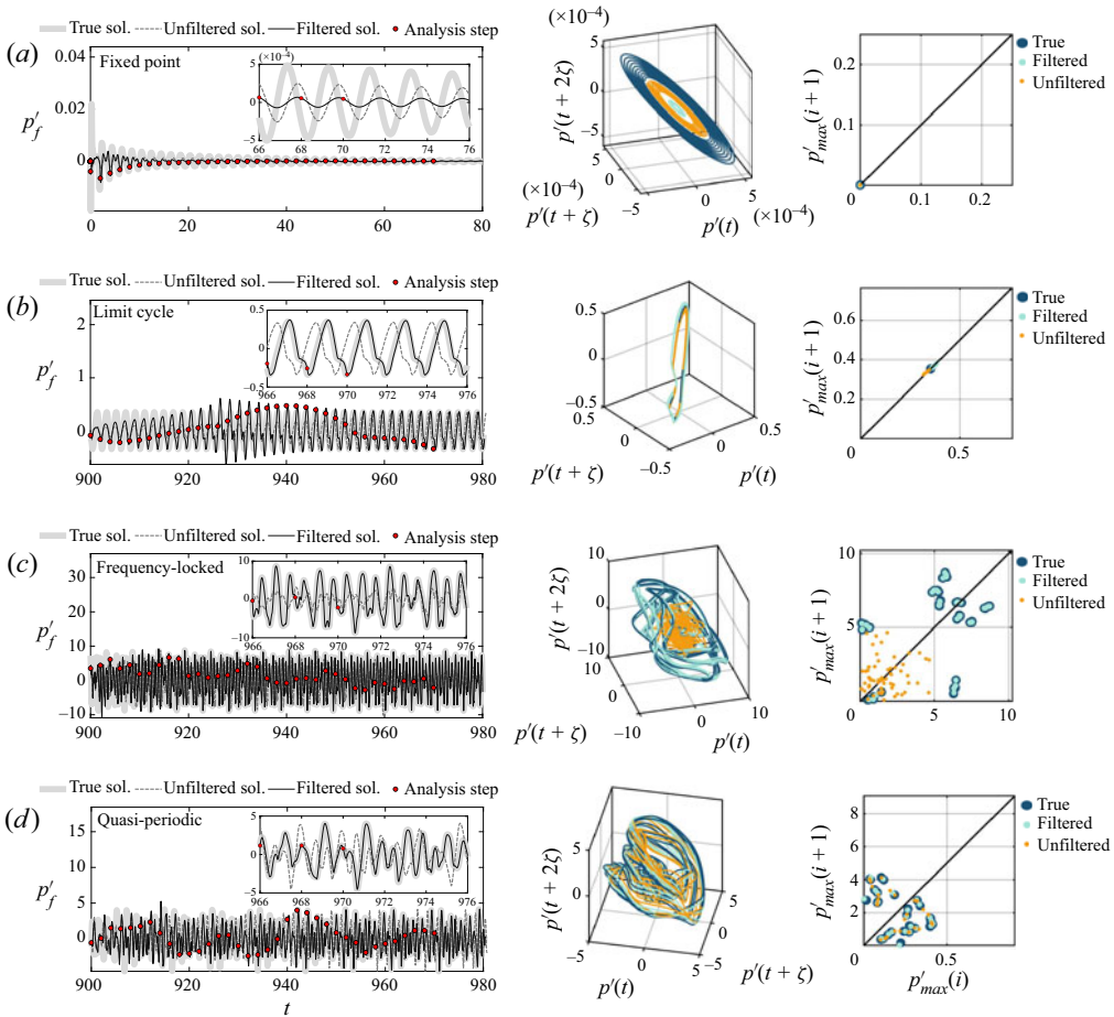
Figure 12. Real-time learning of the state. Assimilation of acoustic pressure from microphones for state estimation of non-chaotic regimes: (a) transient towards a fixed point ( \beta = 0.2 ); (b) limit cycle ( \beta = 0.4 ); (c) frequency-locked ( \beta = 7.7 ); and (d) quasi-periodic ( \beta = 3.6 ). Left-hand plots: true pressure oscillations at the flame location (light grey), unfiltered solution (dashed dark grey) and filtered solution (black). The analysis time steps are indicated with red circles. Centre and right-hand plots: phase portrait and first return map of the true (dark blue), filtered (light blue) and unfiltered (orange) solutions. Here, m = 10 , \sigma_{mic} = 0.01 and \Delta t_{analysis} = 2 .
