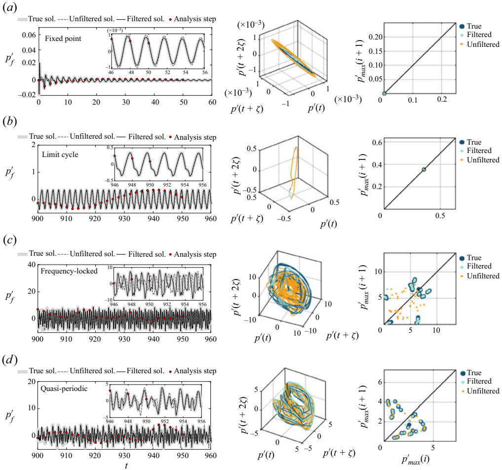
Figure 8. Real-time learning of the state. Assimilation of acoustic modes for state estimation of non-chaotic regimes: (a) transient towards a fixed point ( \beta = 0.2 ); (b) limit cycle ( \beta = 0.4 ); (c) frequency-locked ( \beta = 7.7 ); and (d) quasi-periodic ( \beta = 3.6 ). Left-hand plots: true pressure oscillations at the flame location (light grey), unfiltered solution (dashed dark grey) and filtered solution (black). The analysis time steps are indicated with red circles. Centre and right-hand plots: phase portrait and first return map of the true (dark blue), filtered (light blue) and unfiltered (orange) solutions. Here, m = 10 , \sigma_{frac} = 0.25 and \Delta t_{analysis} = 2 .
