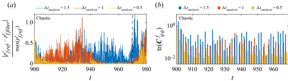
Figure 18. Assimilation of acoustic modes for state estimation of a chaotic regime. Performance metrics. Effect of the assimilation frequency. (a) Relative difference between the filtered solutions and truth. (b) The trace of the ensemble covariance. The dashed vertical line indicates when data assimilation ends. Here, \beta = 7.0 , m = 10 and \sigma_{frac} = 0.25 .
