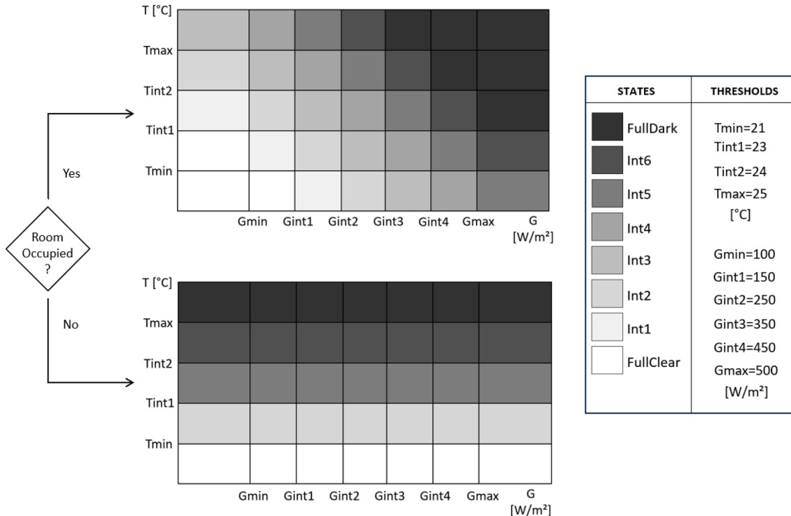
Fig. 6. Diagram representing the logic of the RBC algorithm controlling the electrochromic windows in the study. To the right, the legend includes the names corresponding to the eight tinting states, as well as the internal temperature (T) and incident irradiance on the window (G) thresholds.
