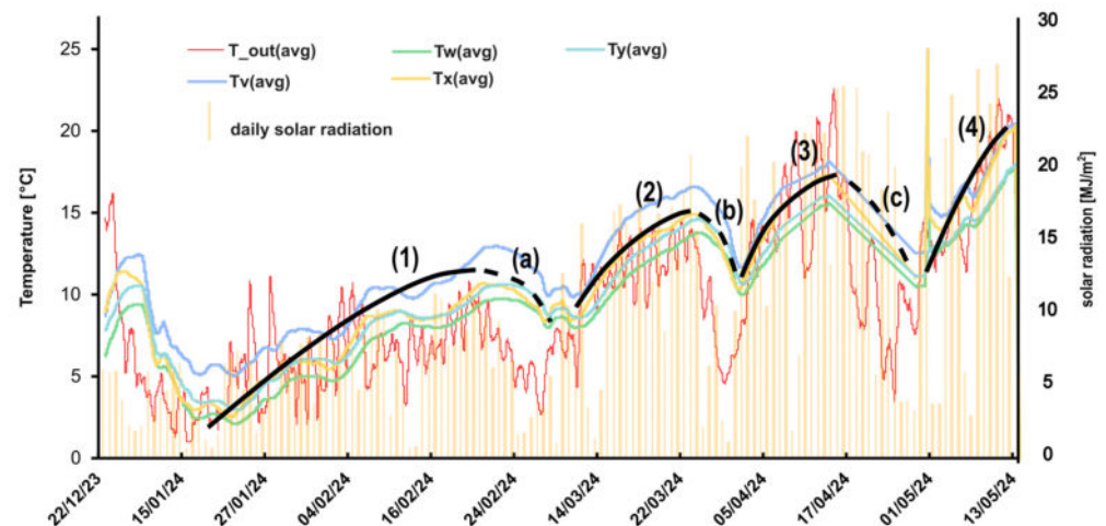
Figure 8. Temperature curves for the setting period.
