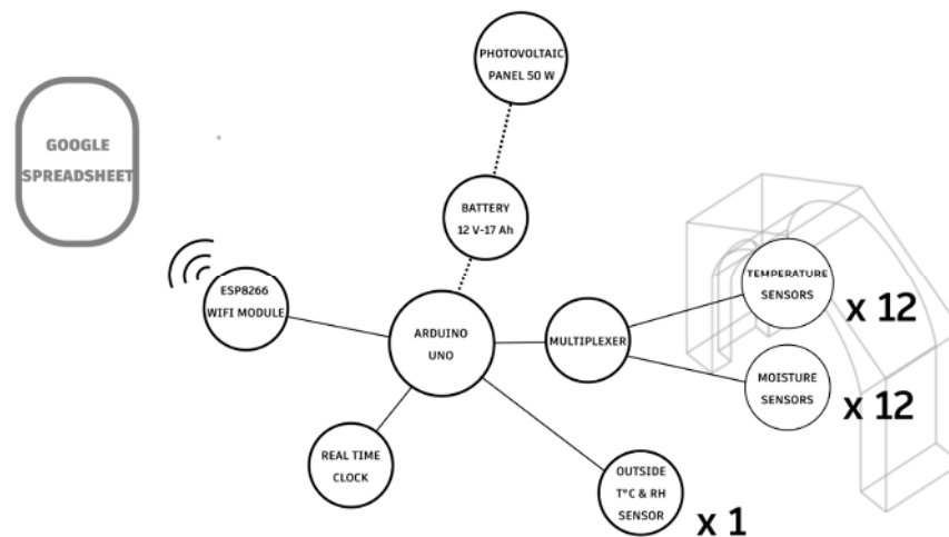
Figure 1. Data acquisition system.
