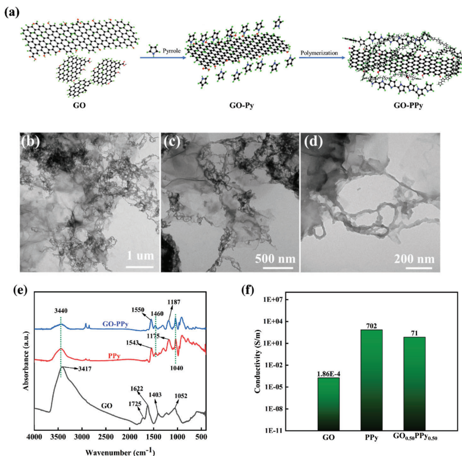
Figure 1. a) Schematic illustration of the assembling mechanism of PPy onto GO in the GO z PPy w samples; b-d) TEM images of GO 0.50 PPy 0.50 ; e) FT-IR spectra of GO, PPy and GO 0.50 PPy 0.50 ; f) electrical conductivity of GO, PPy and GO 0.50 PPy 0.50 .
