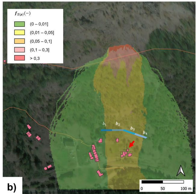
Fig. 3 Study case: a identification of the source area (orange), barrier location (blue line), and of the element at risk (red arrow); b reach probability f_2(\mu) . The case of V^* = 5m^3 is considered
