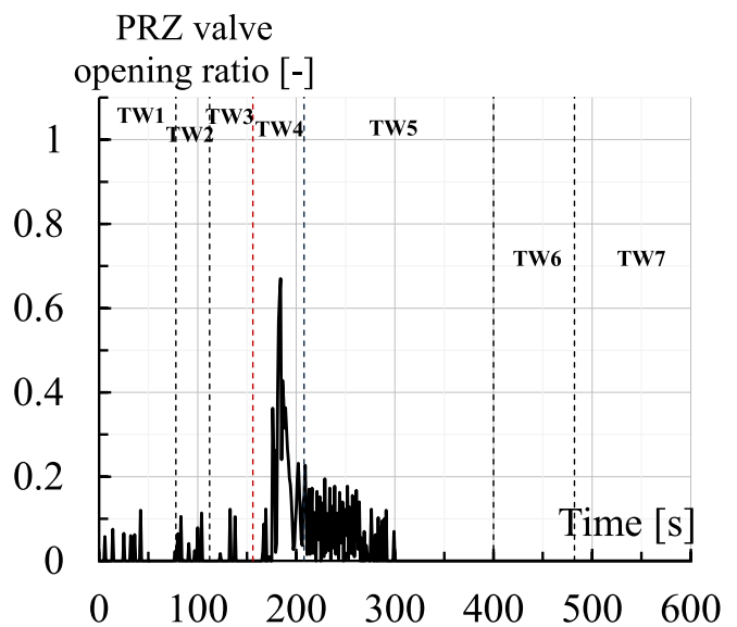
Fig. 19. Pressurizer venting valve opening ratio.
