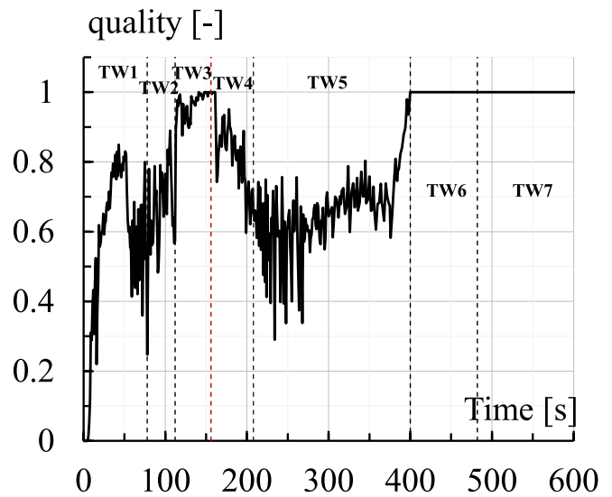
Fig. 18. Average quality in the MHX (water side).
