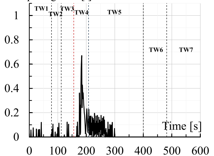
Fig. 19. Pressurizer venting valve opening ratio.
