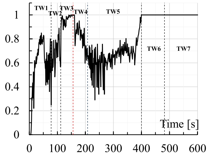
Fig. 18. Average quality in the MHX (water side).
