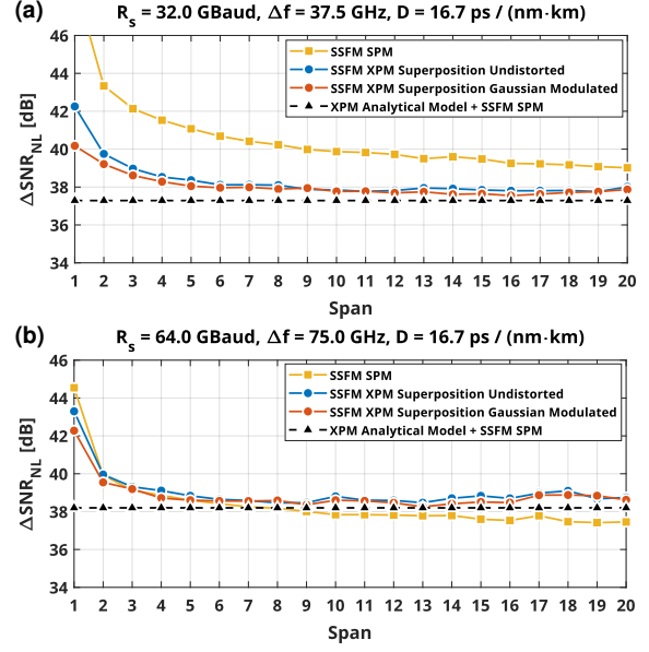
Fig. 3: The SNR NL span-by-span increments, \Delta SNR NL , for: (a) a widespread use case and (b) a realistic high symbol rate transmission scenario. A full-spectrum simulation is compared to a superposition of all constituent pump-and-probe simulations, for both predistortion cases.
