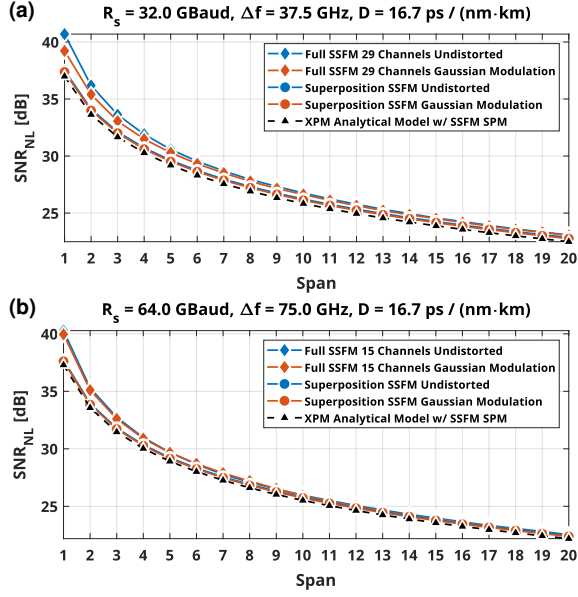
Fig. 2: The SNR NL accumulations for: (a) a widespread use case, and (b) a realistic high symbol rate transmission scenario. A full-spectrum simulation is compared to a superposition of all constituent pump-and-probe simulations, for both predistortion cases.
