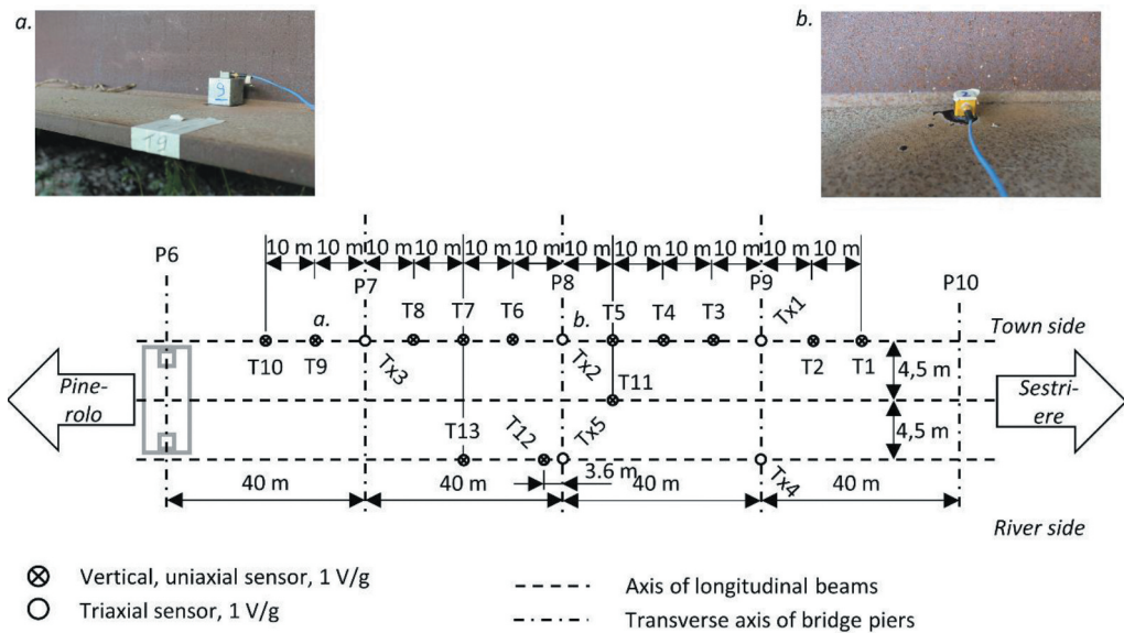
Figure 4. The sensor layout for the bridge deck, including a picture of the capacitive uniaxial (a) and piezoelectric triaxial (b) Accelerometers.
