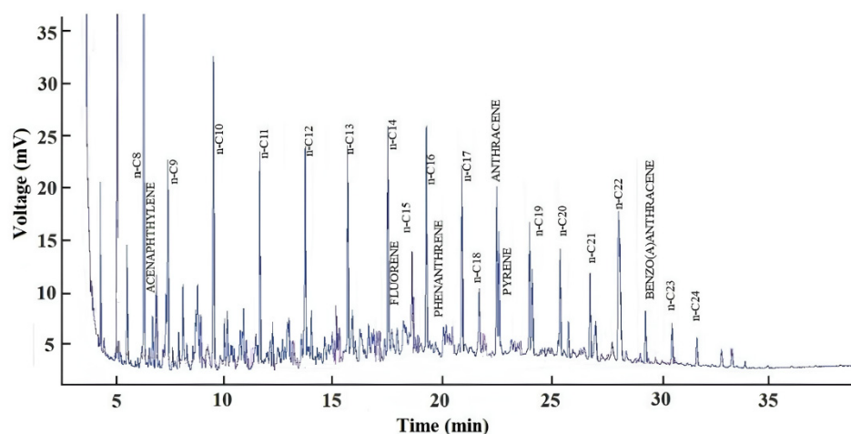
Figure 2. Chromatogram of the commercial diesel oil used in the study.
