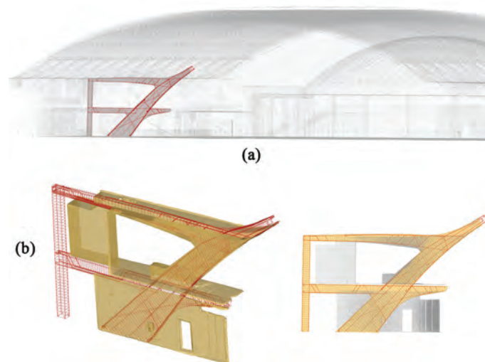
8a 2.4: (a) Integration of the extrados of the P12 pillar module in the reality-based point cloud. (b) 3D models of the internal structural elements developed from the design phase.
