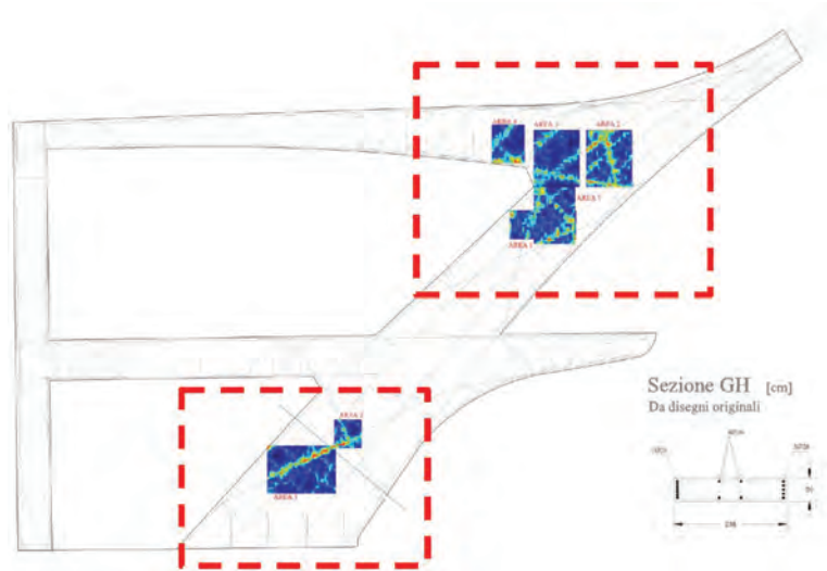
8a 2.3: Overlapping of the reinforcement detected by georadar with respect to the reinforcement as designed by Pier Luigi Nervi.
