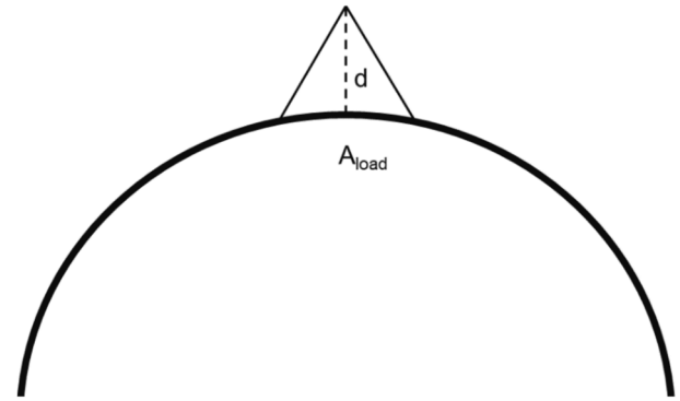
Fig. 4. Basic scheme of a rock block prone to fall from the crown of an underground cavity in a 2D vertical section perpendicular to the cavity axis.
