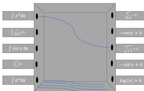
Fig. 2: A scheme of the first challenge. Each indefinite integral must be connected to the correct antiderivative.
